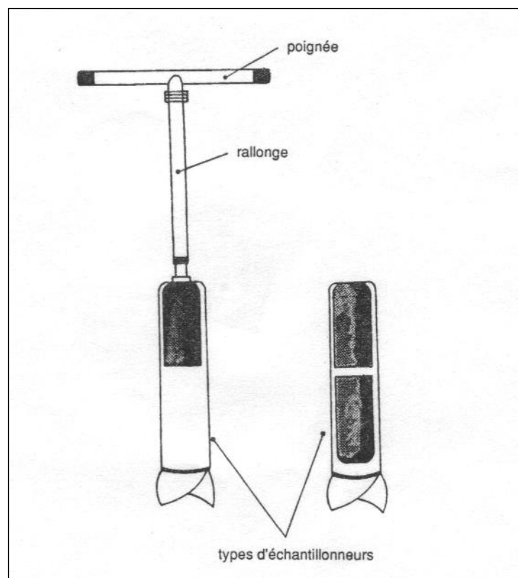
Figure 1 : Tarière manuelle
