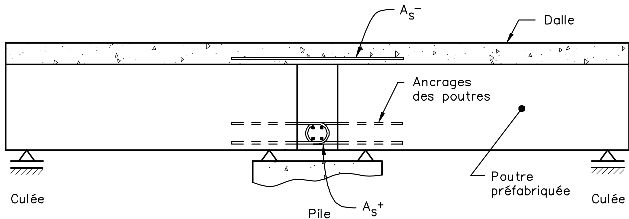
Figure 8.3-4 Structure semi-continue
