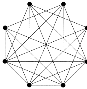
Figure 5: The graph C_4 \cup 4 \times K_1 .
