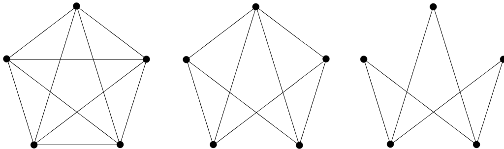
Figure 1: Three extremal graphs on 5 vertices for the bound of Theorem 2.
