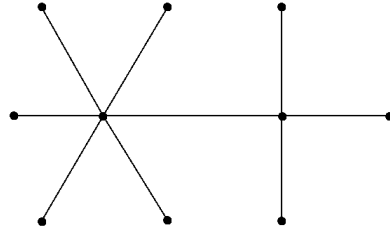
Figure 3: The double star S_{6,4} .
