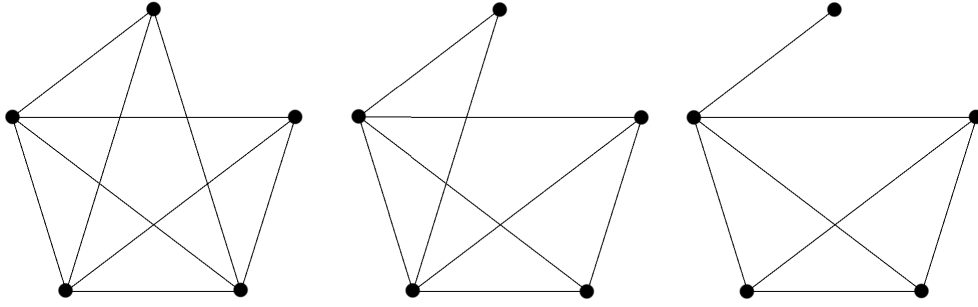
Figure 2: All graphs for the bound of Theorem 6 on 5 vertices.
