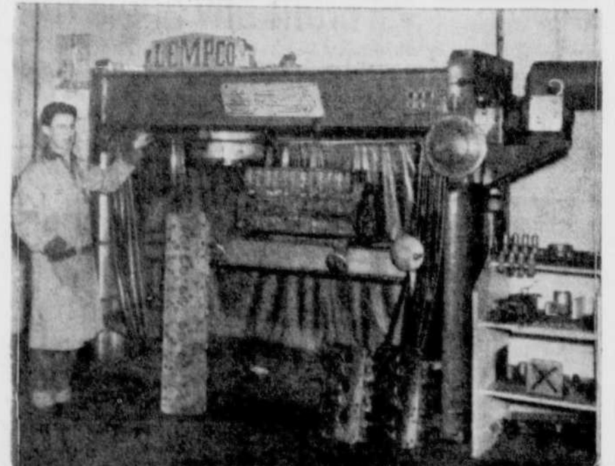
Cleophas Labbe, operator of the Lempco wet-grinding machine used to reface motor blocks and heads of all kinds, including Diesel industrial units... a specialty of our organization. The function of this machine is to regrind the head and block within a thousandth of an inch for a perfect fit.
