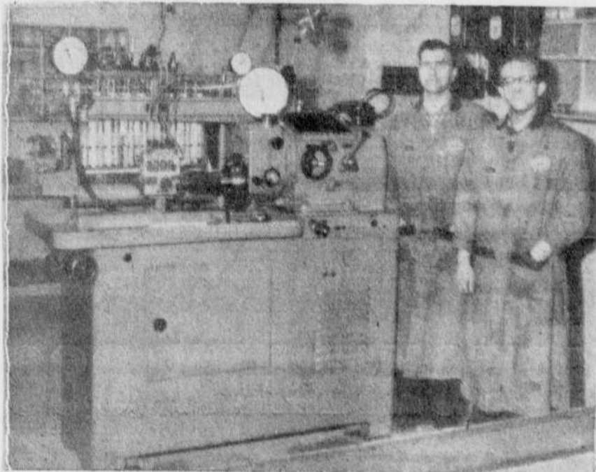
The "Bosch" injection pump calibrator is supervised by Yves Barbier, who also repairs injectors. This German-made precision machine is used in the reconditioning of pumps and injectors for Diesel motors.
