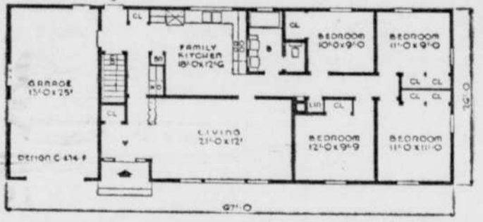
A SMALL HOUSE PLANNING BUREAU DESIGN NO. C-474-F
