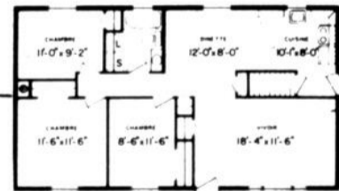
B-1008-C 24'-0" x 42'-0"
