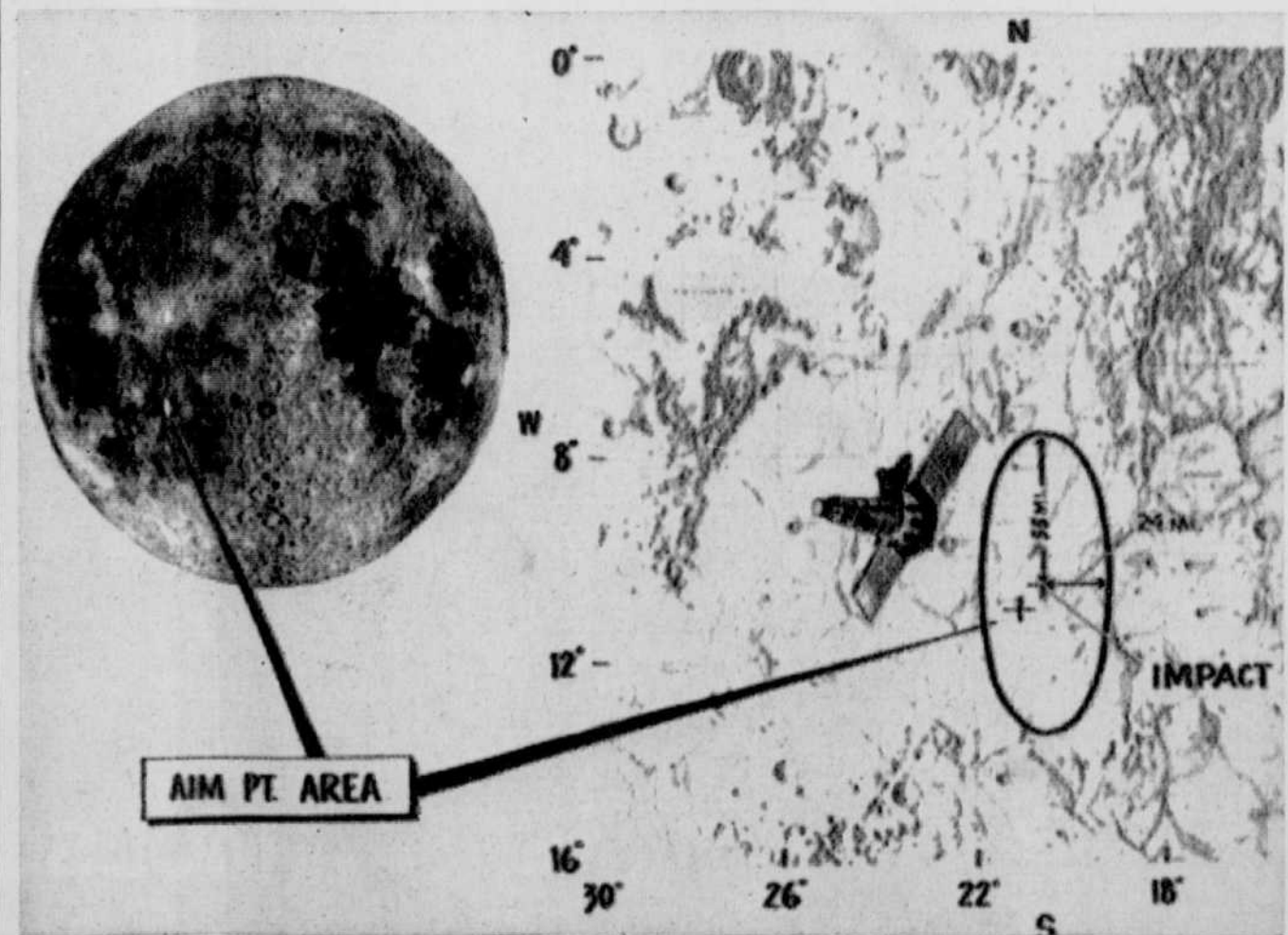
TARGET FOR RANGER 7 — Oval-shaped area is the Sea of Clouds region on the moon in which Ranger 7 made impact this morning. NASA officials reported splendid
