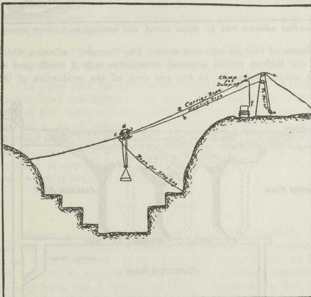
Diagram of quarrying asbestos rock by open pit, and hoisting by cable derrick.
