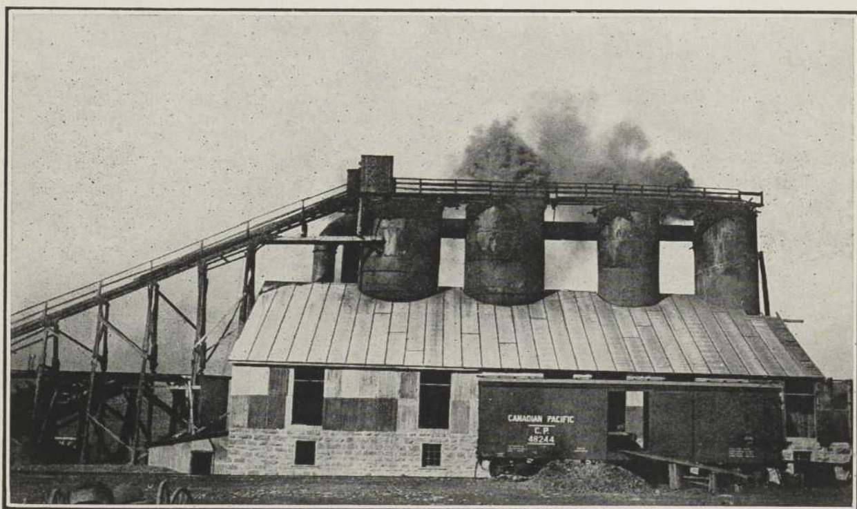
A battery of modern lime kilns at Deschambault.
