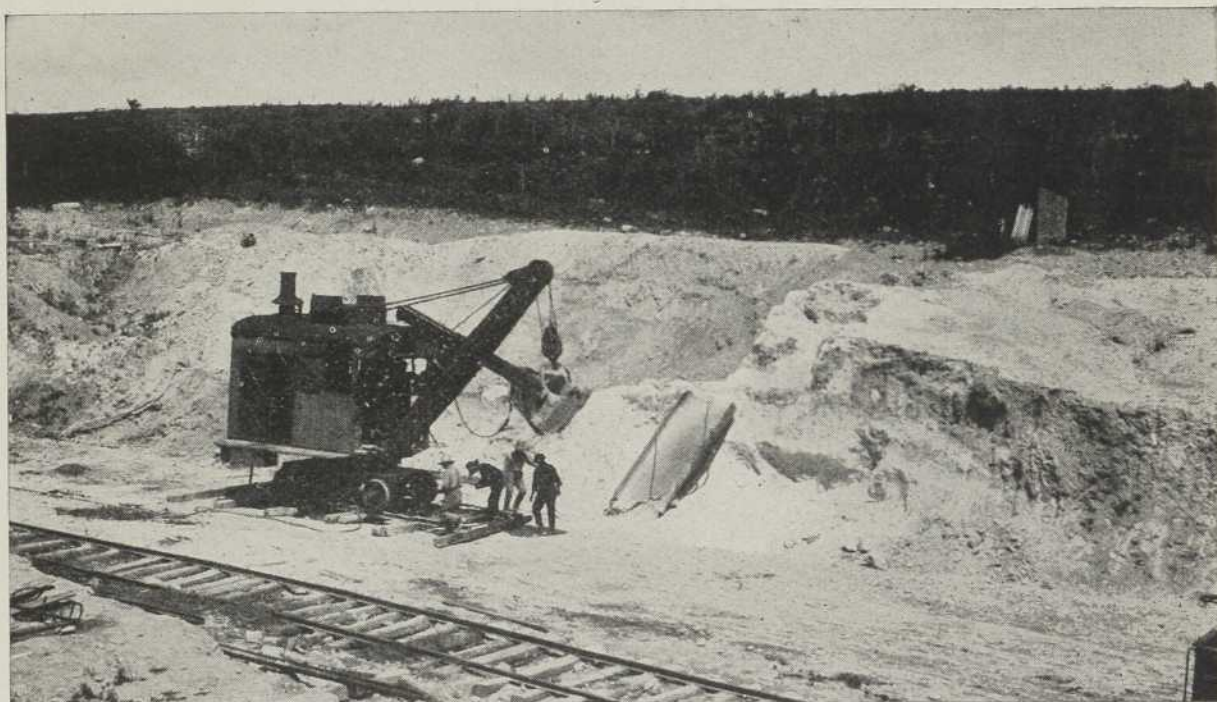
Removing overburden from a deposit of china-clay in Amherst township.
