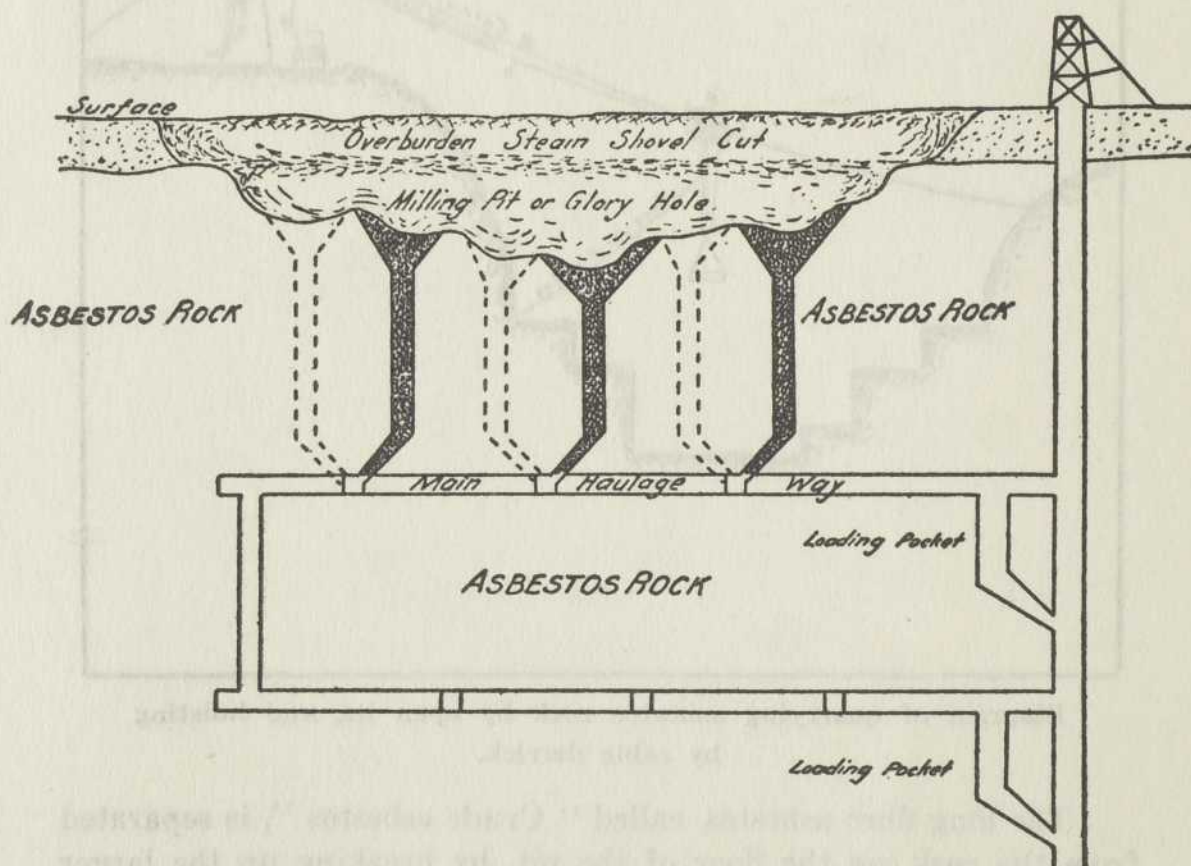
Mining asbestos rock by "Milling" or "Glory-hole" method. The two levels are 175 feet apart and shaft 515 feet deep.
