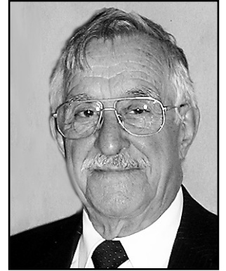
RODRIGUE, Bernard 1924 - 2011
