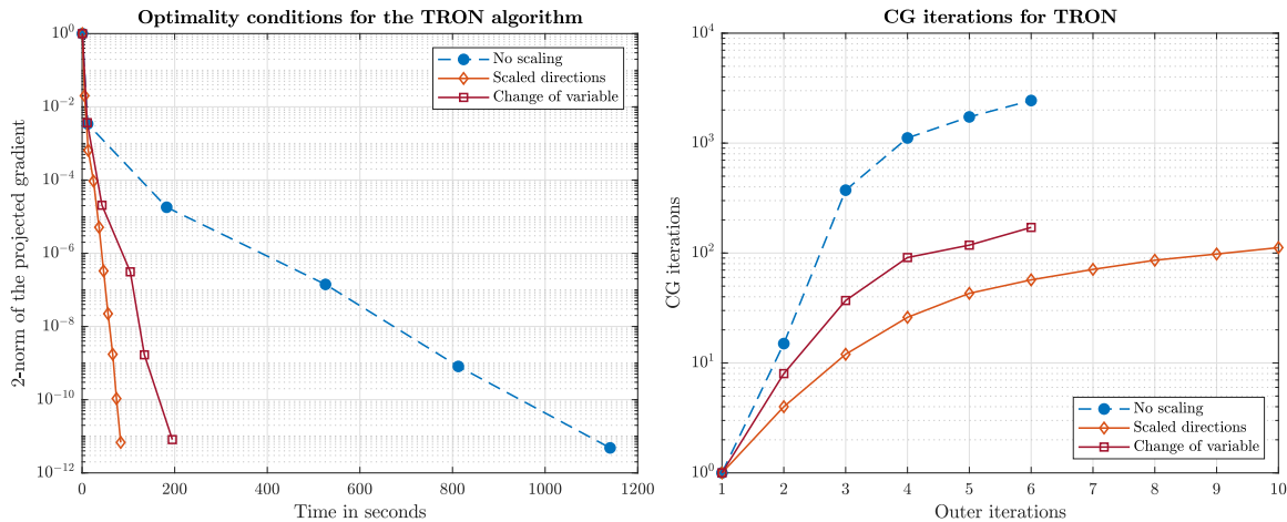
Figure 4: Convergence results for TRON on (25).
