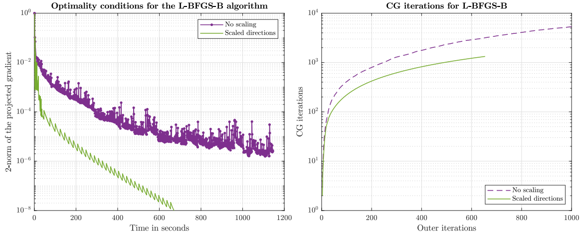
Figure 3: Convergence results for L-BFGS-B on (25).
