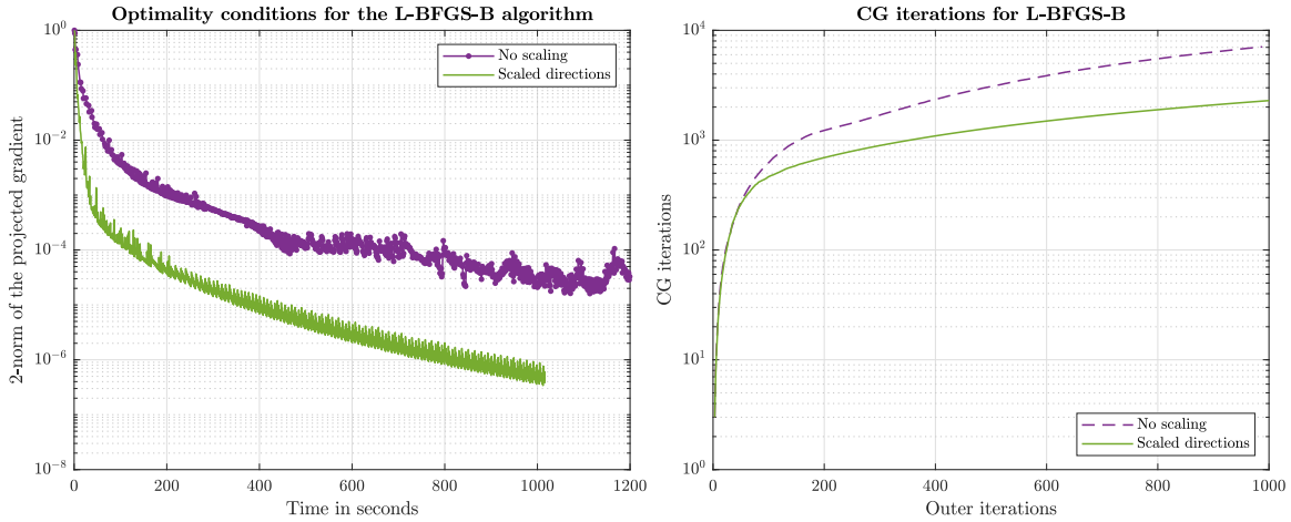
Figure 5: Convergence results for L-BFGS-B on (26).
