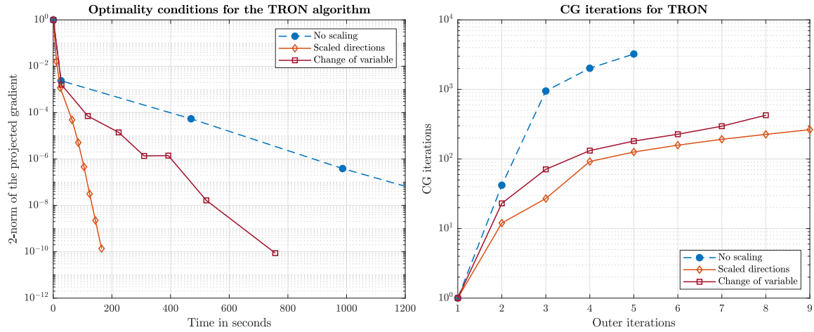
Figure 6: Convergence results for TRON on (26).
