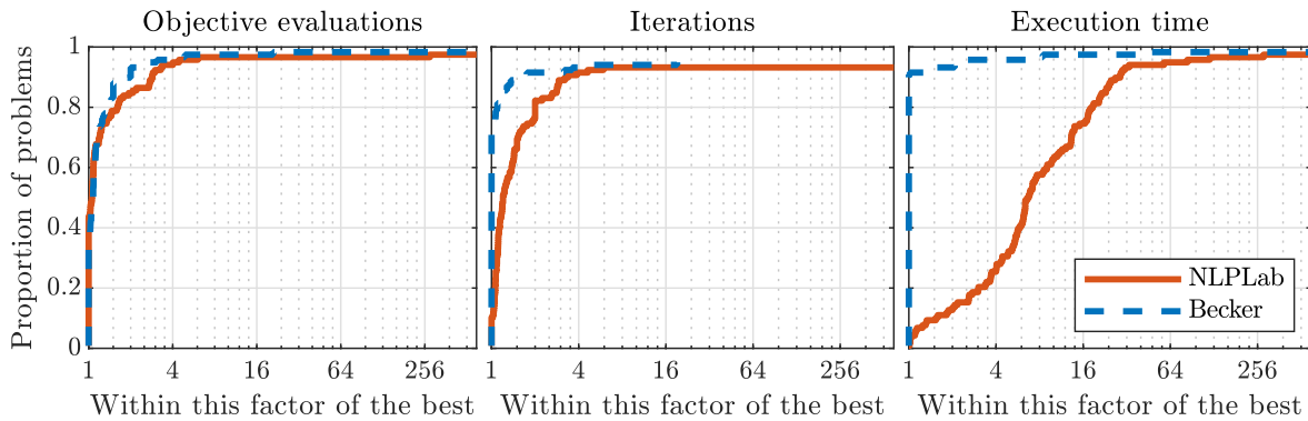
Figure 1: Log-scale performance profiles of our MATLAB implementation versus the C interface. The values compared are the number of objective evaluations (left), the number of iterations (middle) and the execution time (right).
