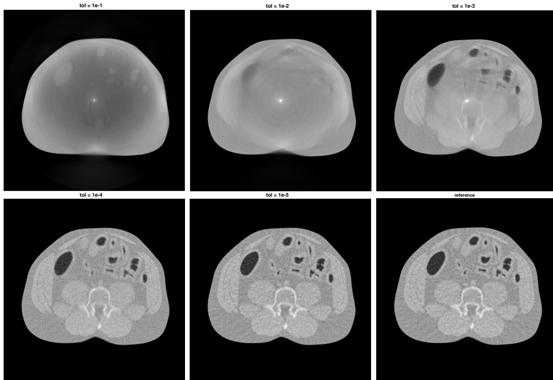
Figure 8: Images obtained with SPG for several tolerances. The reference image is obtained with TRON with tolerance 10^{-10} .
