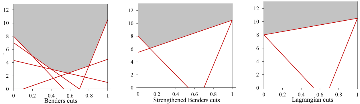
Figure 1 Performance of different cuts in cutting the solution space of LP master problem
