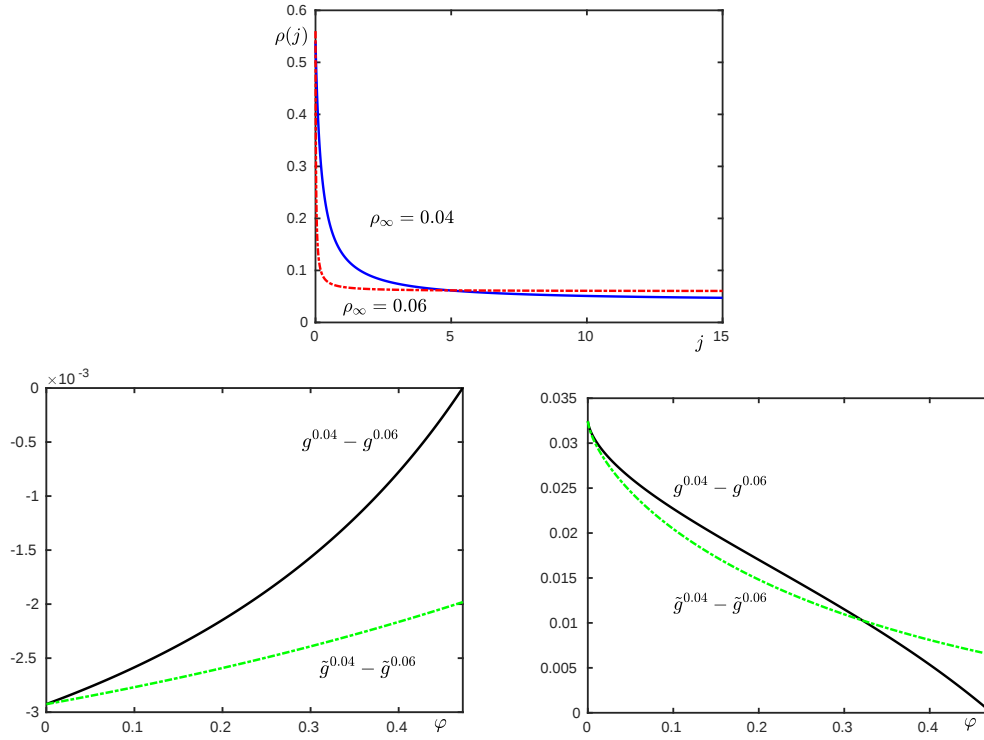
Figure 5: Effect of \rho_\infty . Bottom left \sigma = 0.8 ; bottom right \sigma = 1.5 .
