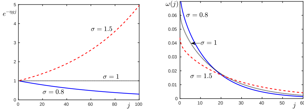
Figure 1: Future marginal effects in utility (left); and weights \omega(j) (right).
