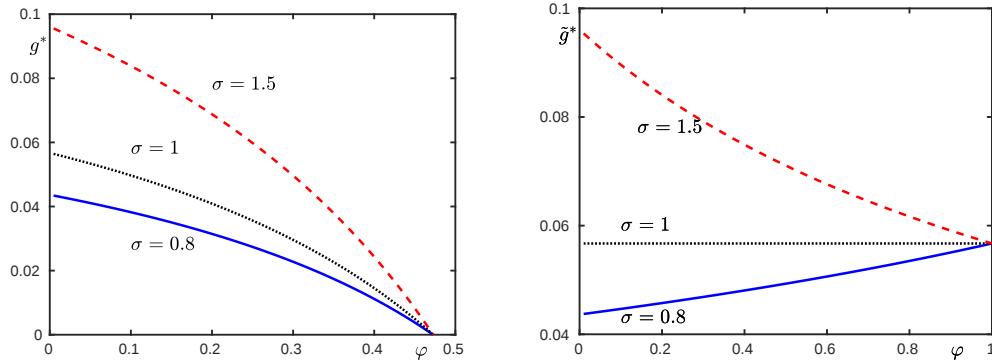
Figure 3: Sensitivity of g^* (left) and \tilde{g}^* (right) w.r.t. \sigma and \varphi .
