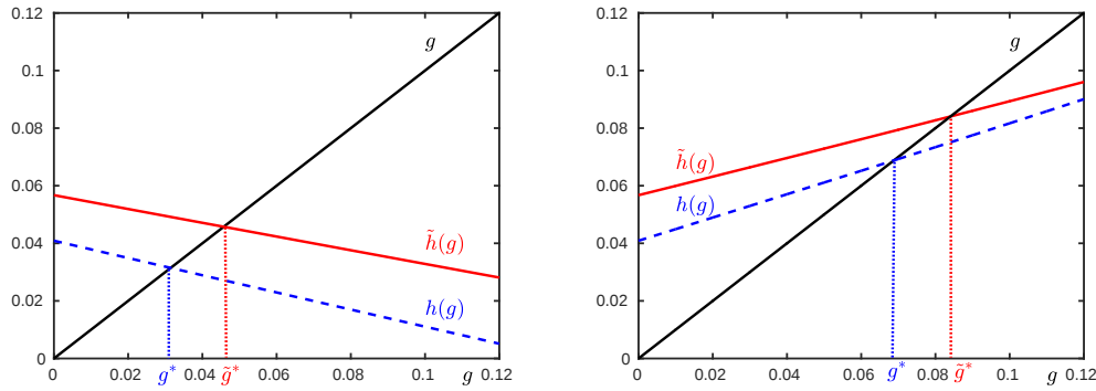
Figure 2: Equilibrium growth rates, g^* and \tilde{g}^* , for \sigma < 1 (left) \sigma > 1 (right).
