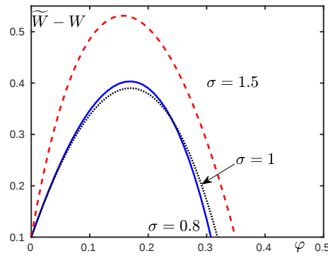
Figure 6: \widetilde{W}(K_t, K_t) - W(K_t) with respect to \varphi .
