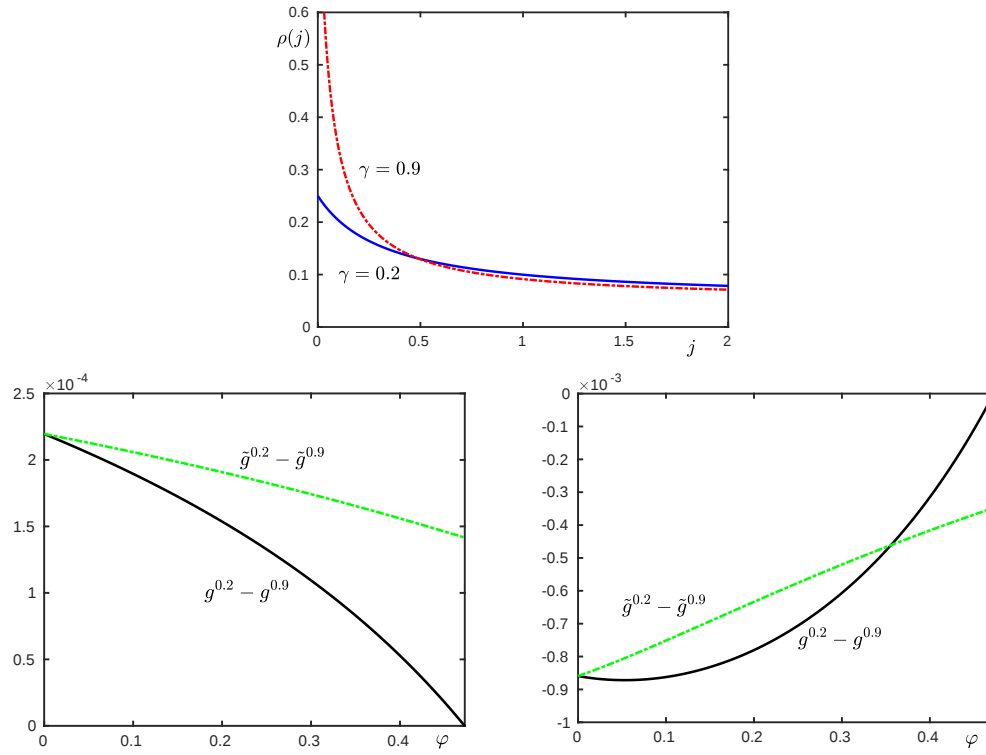
Figure 4: Effect of \gamma . Bottom left \sigma = 0.8 ; bottom right \sigma = 1.5 .
