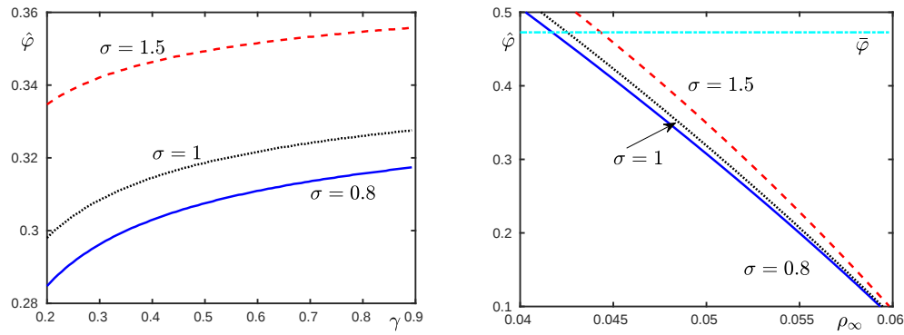
Figure 7: Effect of \gamma (left) and \rho_\infty (right) on \hat{\varphi} .
