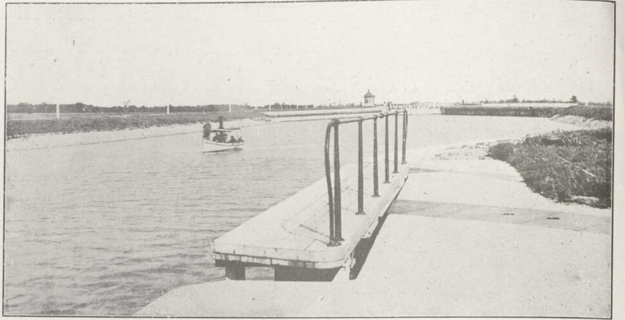
The basin between guard gate and lock No. 4 on the Soulanges Canal.
