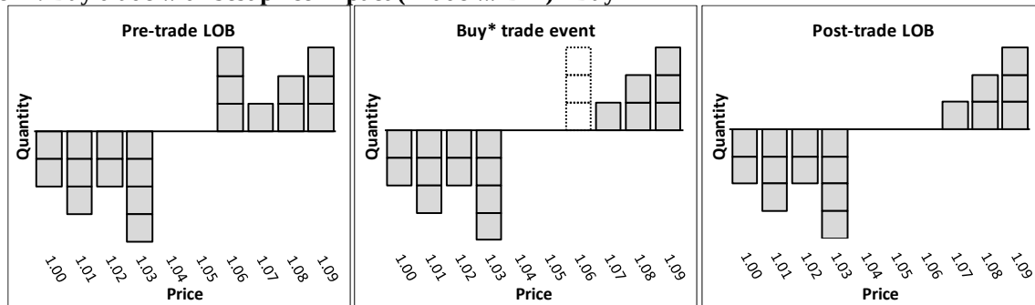
Figure 2 Fictional events examples and their LOB effects
