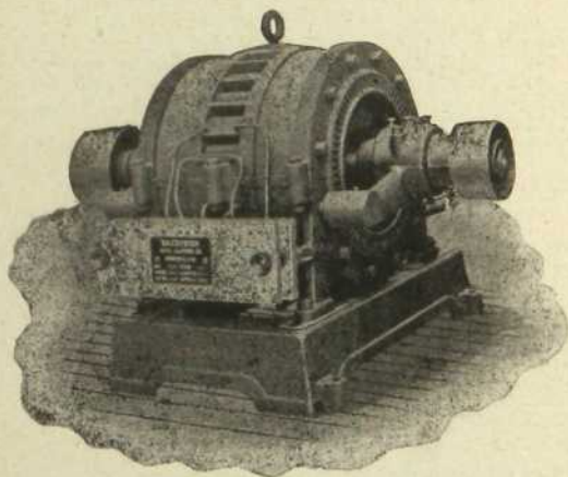
40 K. W. Generator, Wound for 150 Volts.
