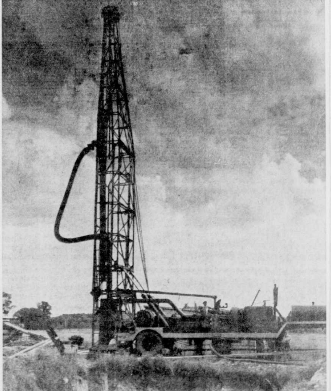
NEW WATER SUPPLY — Seen above is the new Lennoxville Town well, located not far from the old one, on Herring's Farm, just outside the town limits on the Stanstead highway. This new well is part of the plan for augmenting the municipal water supply, and is expected to deliver upwards of 800 gallons of water per minute. The old well delivers about 600 gallons a minute. (Record photo by Gerry Lemay)
