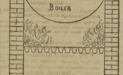
FIG. 1.—FIRING WITH SHAVINGS.
