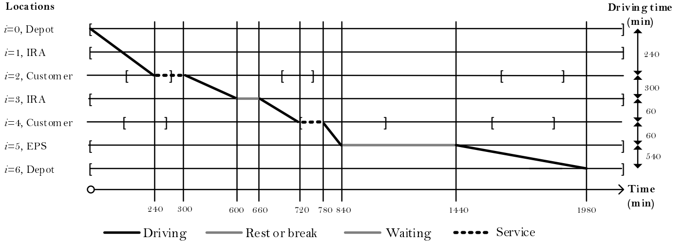
Figure 4: An illustrative example of the TDSP-IO.
