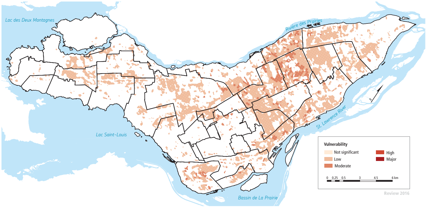
MAP 6.5 VULNERABILITY TO HEAT WAVES IN THE MONTRÉAL AGGLOMERATION
