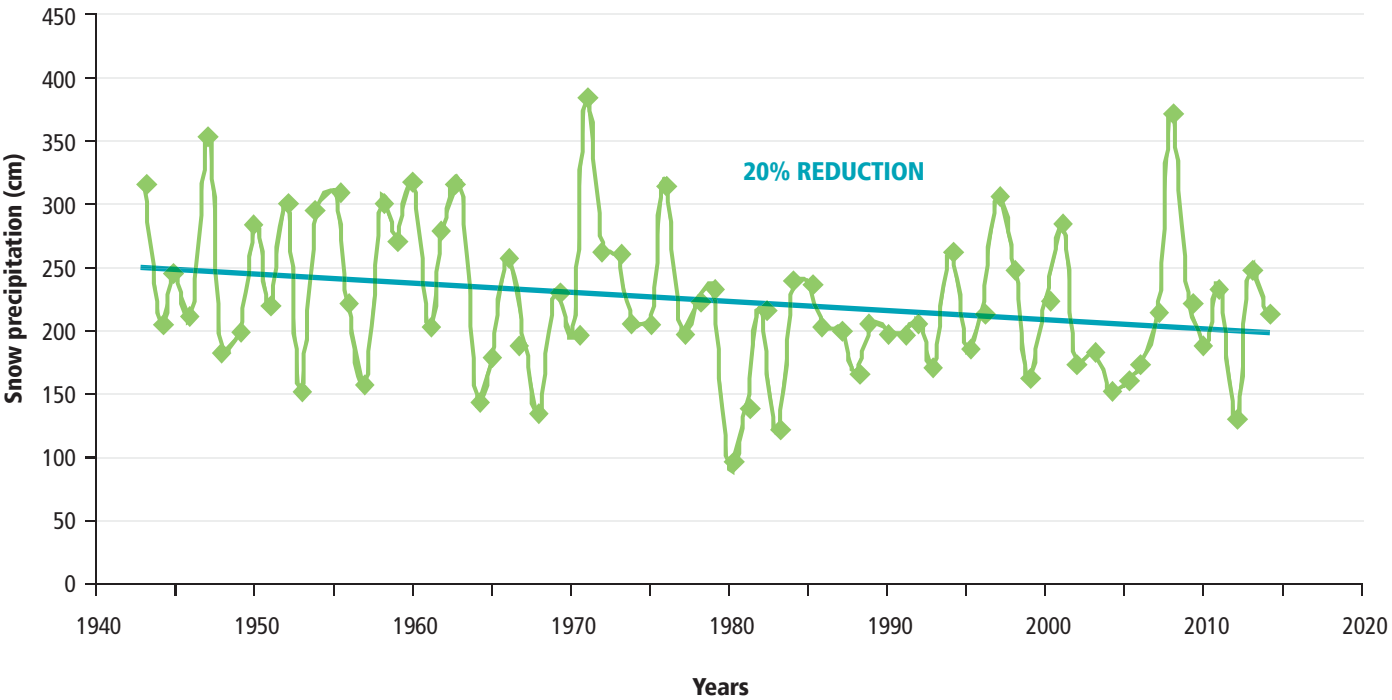
FIGURE 5.4 EVOLUTION OF SNOWFALL AMOUNTS, 1942-2014 Source: Data from the weather station at the Montréal-Trudeau International Airport.
