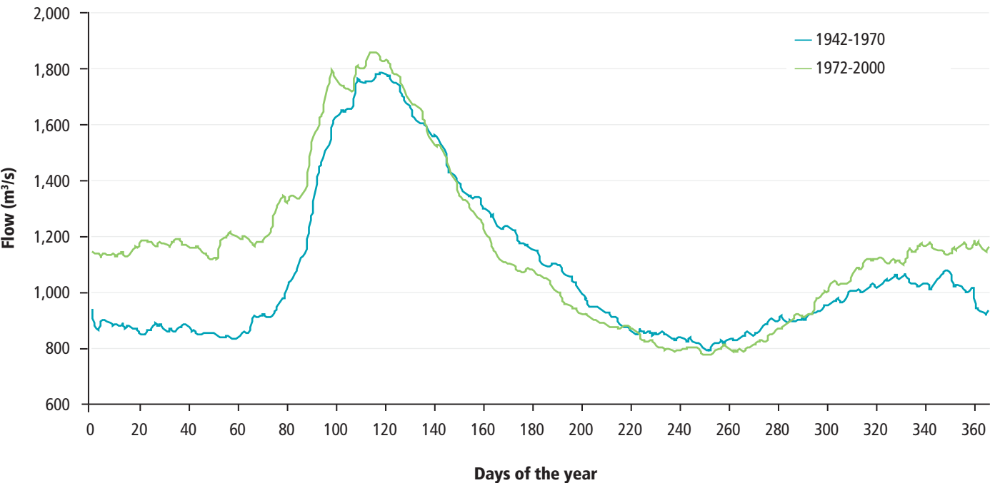
FIGURE 9.2 AVERAGE DAILY FLOW FOR RIVIÈRE DES PRAIRIES
