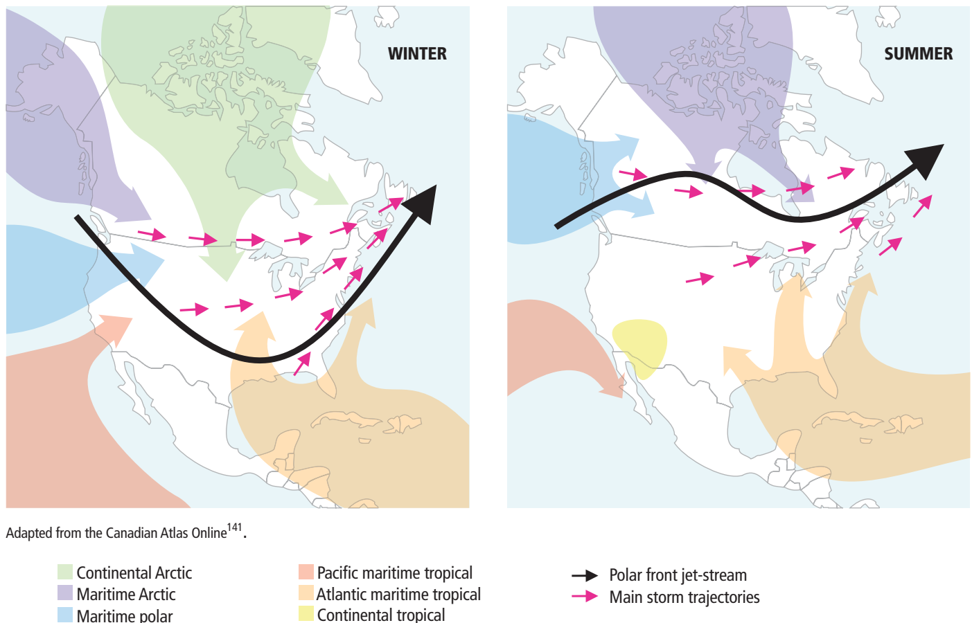
FIGURE 2.3 AIR MASSES THAT INFLUENCE CANADA'S CLIMATE
