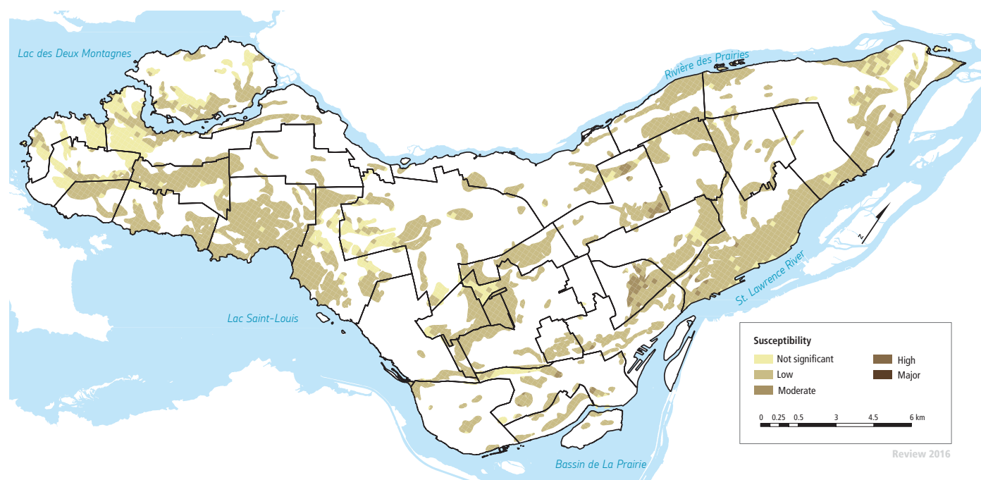
MAP 8.1 TERRITORIAL SUSCEPTIBILITY IN THE AREAS OF THE MONTRÉAL AGGLOMERATION EXPOSED TO SOIL CONTRACTION
