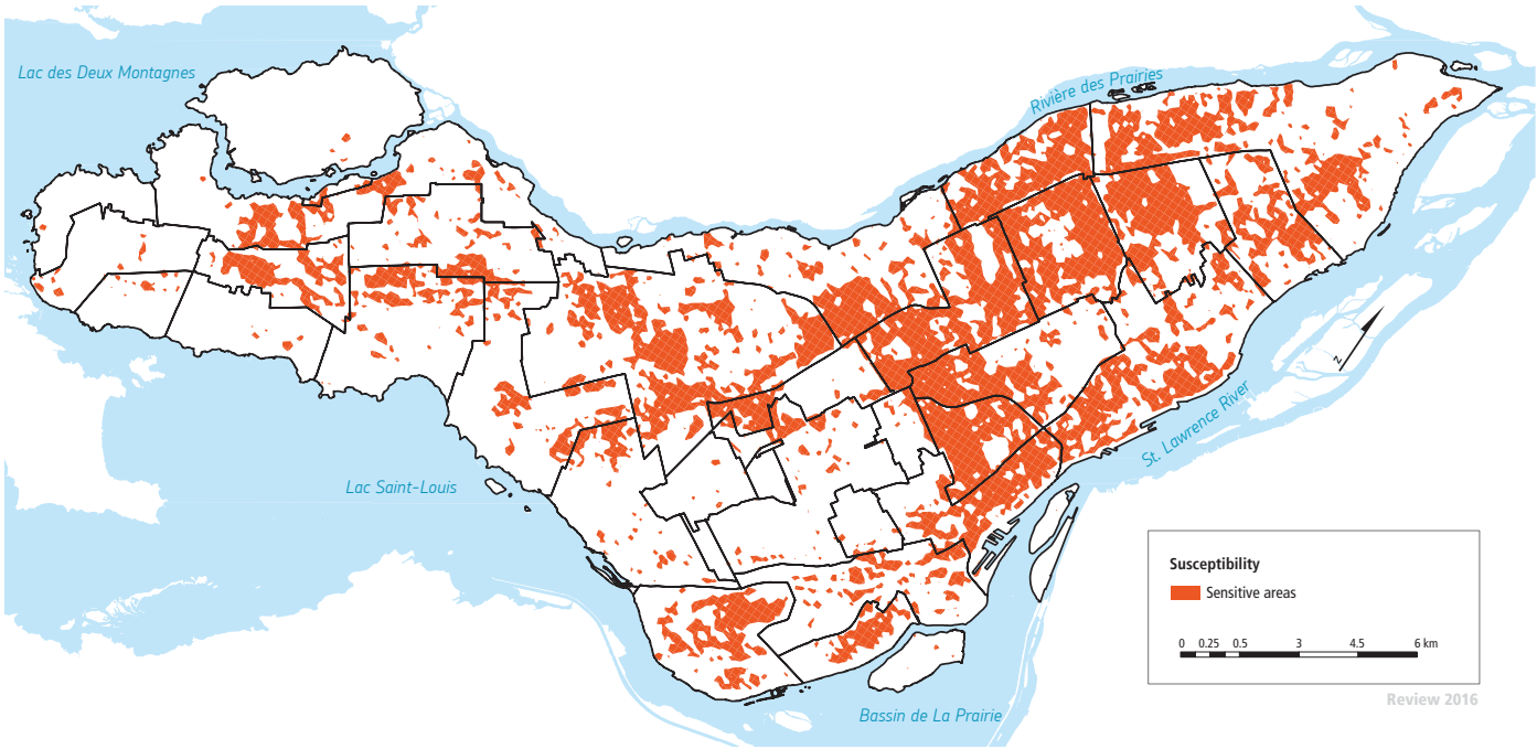
MAP 6.4 INTRA-URBAN HEAT ISLANDS IN THE MONTRÉAL AGGLOMERATION
