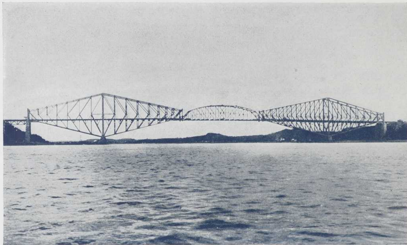
Quebec Bridge Over the St. Lawrence River—Length, 3239 eet . Height above water, 150 feet. Cost, $25,000,000.
