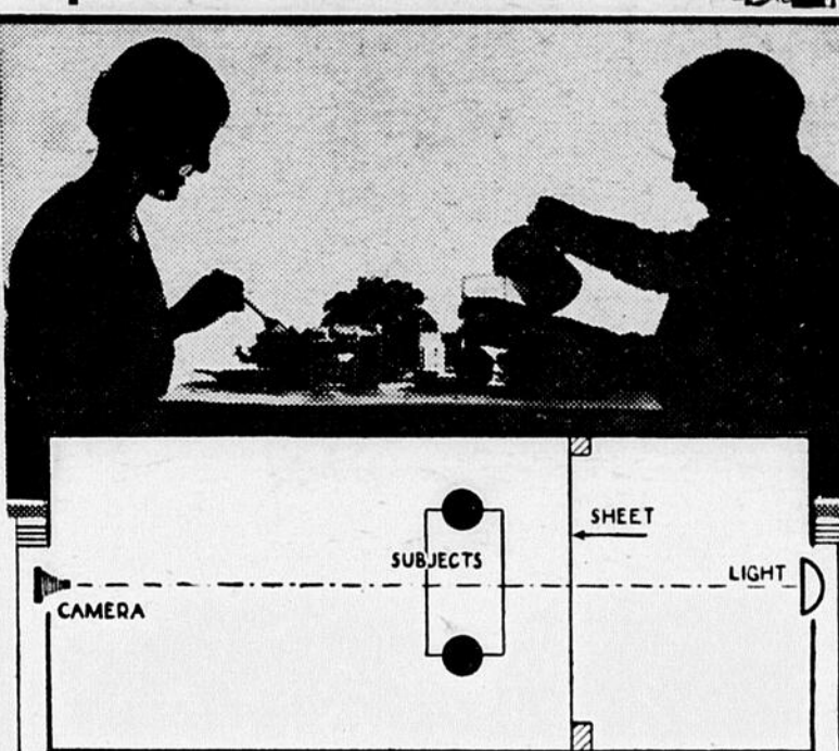
An arched doorway between living and dining rooms, a taut sheet and a bright light —these were the only special requirements for this silhouette. The diagram shows the relative positions of camera, subjects, sheet and light.
