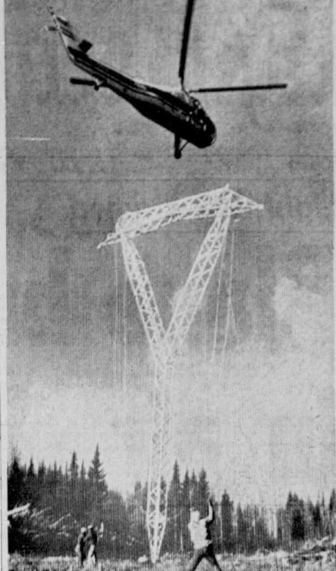
TOWERS IN THE SKY — Giant helicopter overcomes the problems of transporting towers in establishing a 30-mile power transmission line in the rugged foothills country northwest of Rocky Mountain House, Alta. The helicopter, owned by Okanagan Helicopters Limited, flies the special aluminum towers to their sites, where ground crews guide them to their bases and anchor them. The project is being carried out for Calgary Power Limited. (CP Photo)
