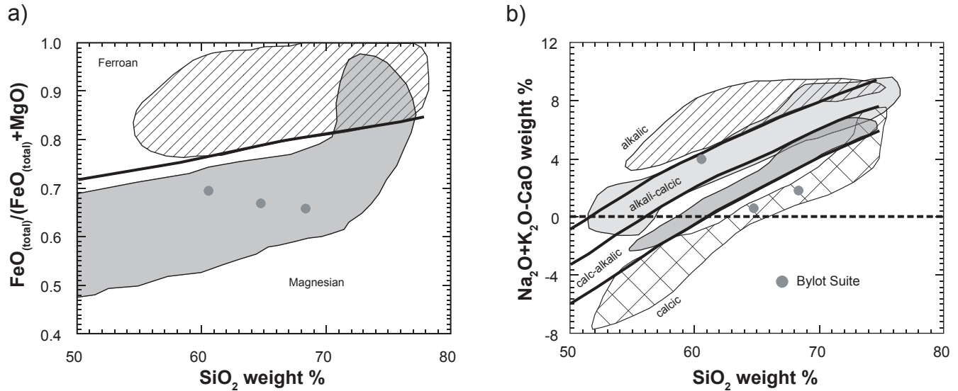
FIGURE 4.7 – TTG series, Bylot Suite: a) classification diagram by Frost et al. (2001), \text{FeO}_{\text{(total)}}/(\text{FeO}_{\text{(total)}}+\text{MgO}) vs \text{SiO}_2 (weight %); b) classification diagram by Frost et al. (2001), \text{Na}_2\text{O}+\text{K}_2\text{O}-\text{CaO} vs \text{SiO}_2 (weight %).
