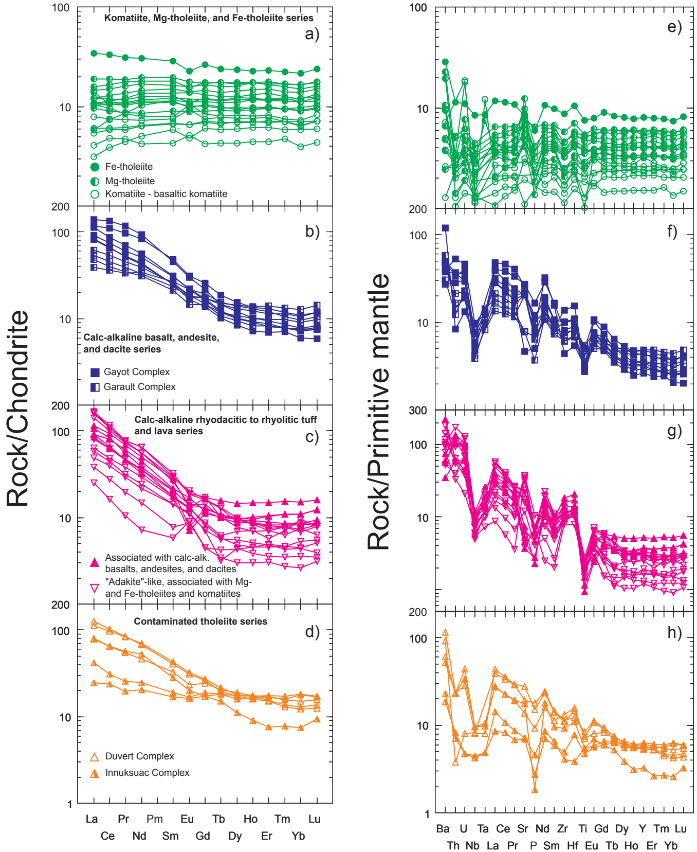
FIGURE 4.3 – Chondrite-normalized REE patterns and primitive mantle-normalized multi-element diagrams for volcanic rocks in the NESF: a) and e) komatiite, Mg-tholeiite, and Fe-tholeiite series; b) and f) calc-alkaline basalt, andesite, and dacite series; c) and g) calc-alkaline rhyodacitic to rhyolitic tuff and lava series; d) and h) contaminated tholeiite series.
