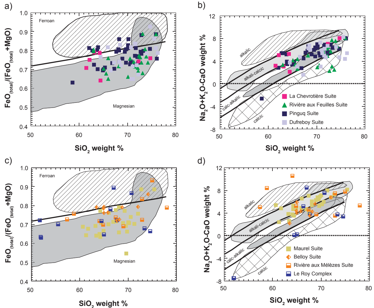
FIGURE 4.9 – GGM series, La Chevrotière, Pingu, Dufrebois, Maurel, and Belloy suites: a) and c) classification diagram by Frost et al. (2001), \text{FeO}_{(\text{total})}/(\text{FeO}_{(\text{total})}+\text{MgO}) vs \text{SiO}_2 (weight %); b) and d) classification diagram by Frost et al. (2001), \text{Na}_2\text{O}+\text{K}_2\text{O}-\text{CaO} (weight %) vs \text{SiO}_2 (weight %).
