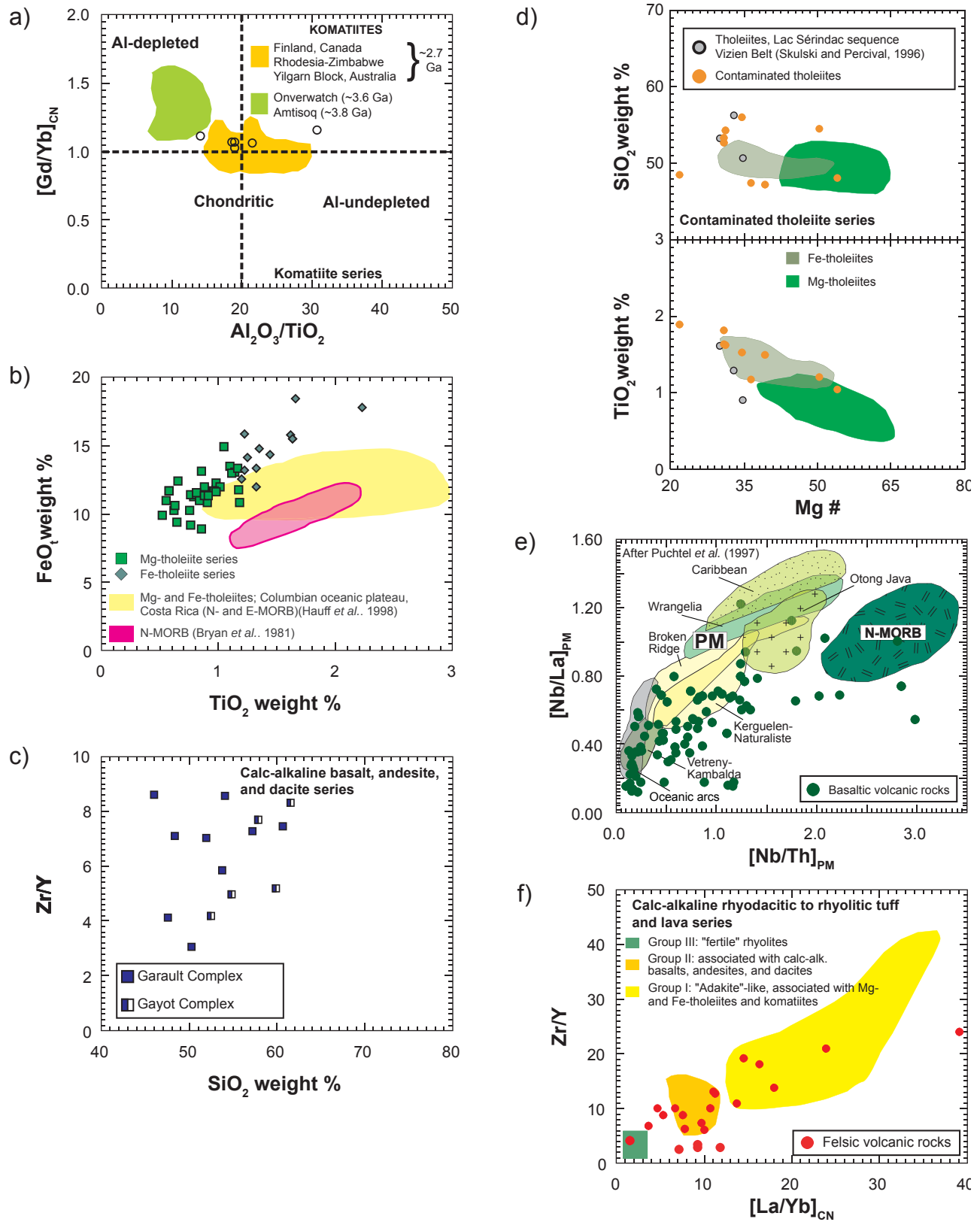
FIGURE 4.4 – Volcanic rocks in the NESF: a) [Gd/Yb]_{CN} vs Al_2O_3/TiO_2 for the komatiite series. Note the chondritic, Al-undepleted nature of NESF komatiites; b) FeO_{total} (weight %) vs TiO_2 (weight %) for the Mg- and Fe-tholeiite series; c) Zr/Y vs SiO_2 (weight %) for the calc-alkaline basalt, andesite, and dacite series; d) TiO_2 (weight %) and SiO_2 (weight %) vs Mg\# for the contaminated tholeiite series. Note TiO_2 and SiO_2 enrichment and high degree of differentiation (i.e. low Mg\# ) of contaminated tholeiites relative to Mg-tholeiites. Tholeiites from the Lac Sérindac sequence (Vizion Belt) are also plotted for comparative purposes; e) [Nb/La]_{PM} vs [Nb/Th]_{PM} for basaltic rocks in the NESF. The latter show similarities with plateau basalts (e.g., Kerguelen-Naturaliste and Broken Ridge) and island arc basalts; f) Zr/Y vs [La/Yb]_{CN} for the calc-alkaline rhyodacitic to rhyolitic tuff and lava series. The three main groups recognized in calc-alkaline felsic volcanic rocks of the NESF are illustrated.
