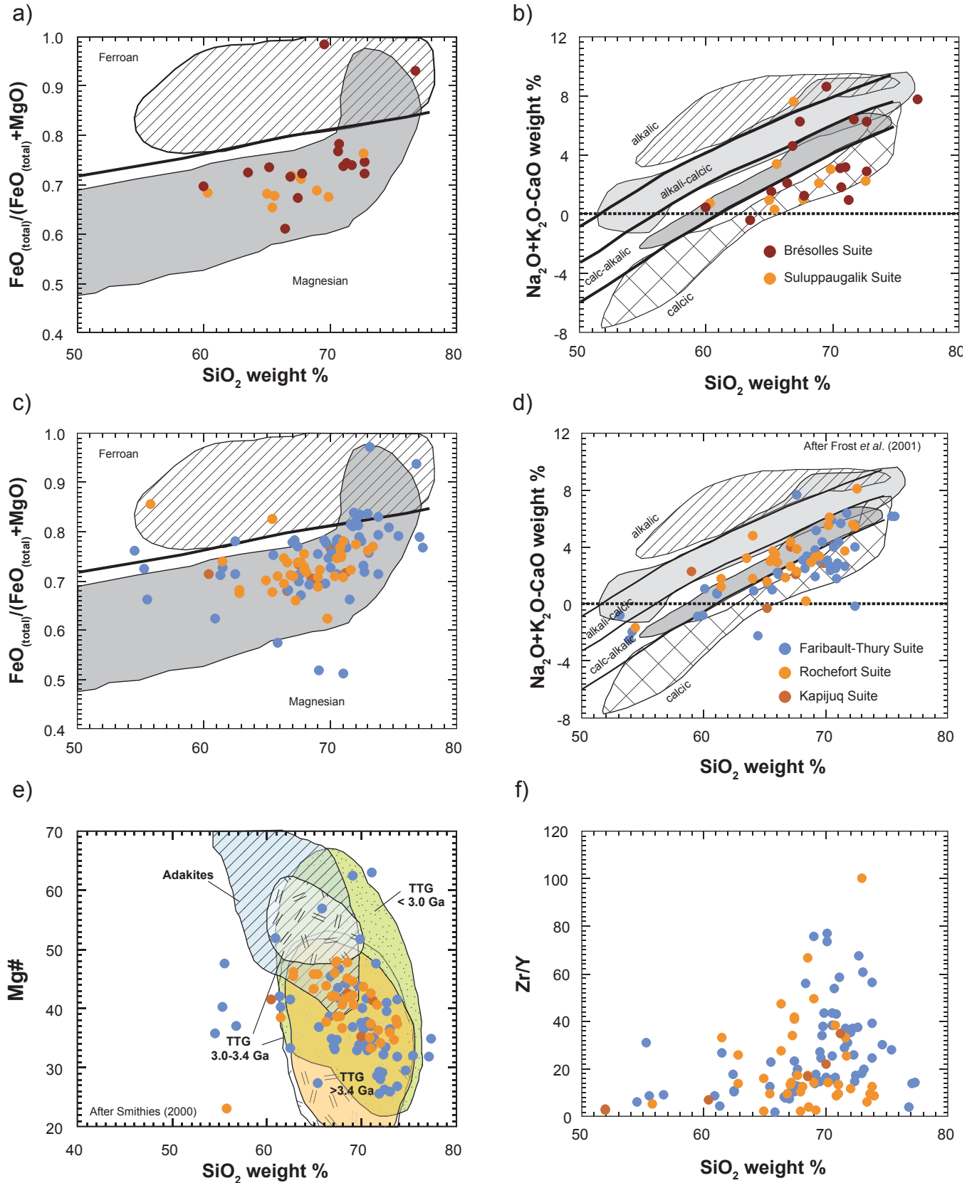
FIGURE 4.6 – TTG series, Brésolles, Suluppaugalik, Faribault-Thury, Rochefort, and Kapijuq suites: a) and c) classification diagram by Frost et al. (2001); FeO (total) /(FeO (total) +MgO) vs SiO 2 (weight %); b) and d) classification diagram by Frost et al. (2001); Na 2 O+K 2 O-CaO (weight %) vs SiO 2 (weight %); e) Mg# vs SiO 2 (weight %) illustrating the absence of adakites in the Faribault-Thury, Rochefort, and Kapijuq plutonic suites (TTG series); f) Zr/Y vs SiO 2 (weight %) showing significant variations in Zr/Y ratios for felsic members of the Faribault-Thury, Rochefort, and Kapijuq suites.
