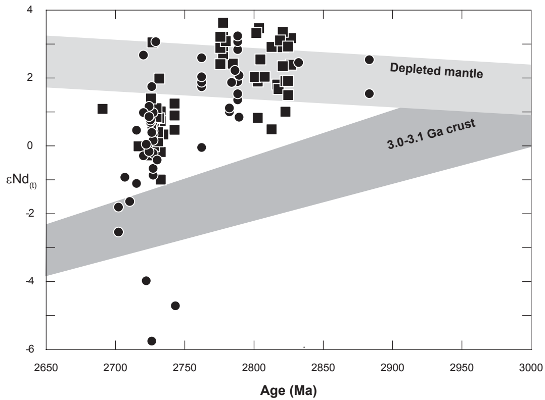
FIGURE 4.15 – \epsilon\text{Nd}(t) vs age of emplacement for: a) felsic rocks, and b) mafic and ultramafic rocks in the NESP. Samples were subdivided based on their location in the Rivière Arnaud or Hudson Bay terranes. The depleted mantle field was calculated using methods described by DePaolo (1982) and Stern et al. (1994). Data derived from compilation by Maurice (2007).
