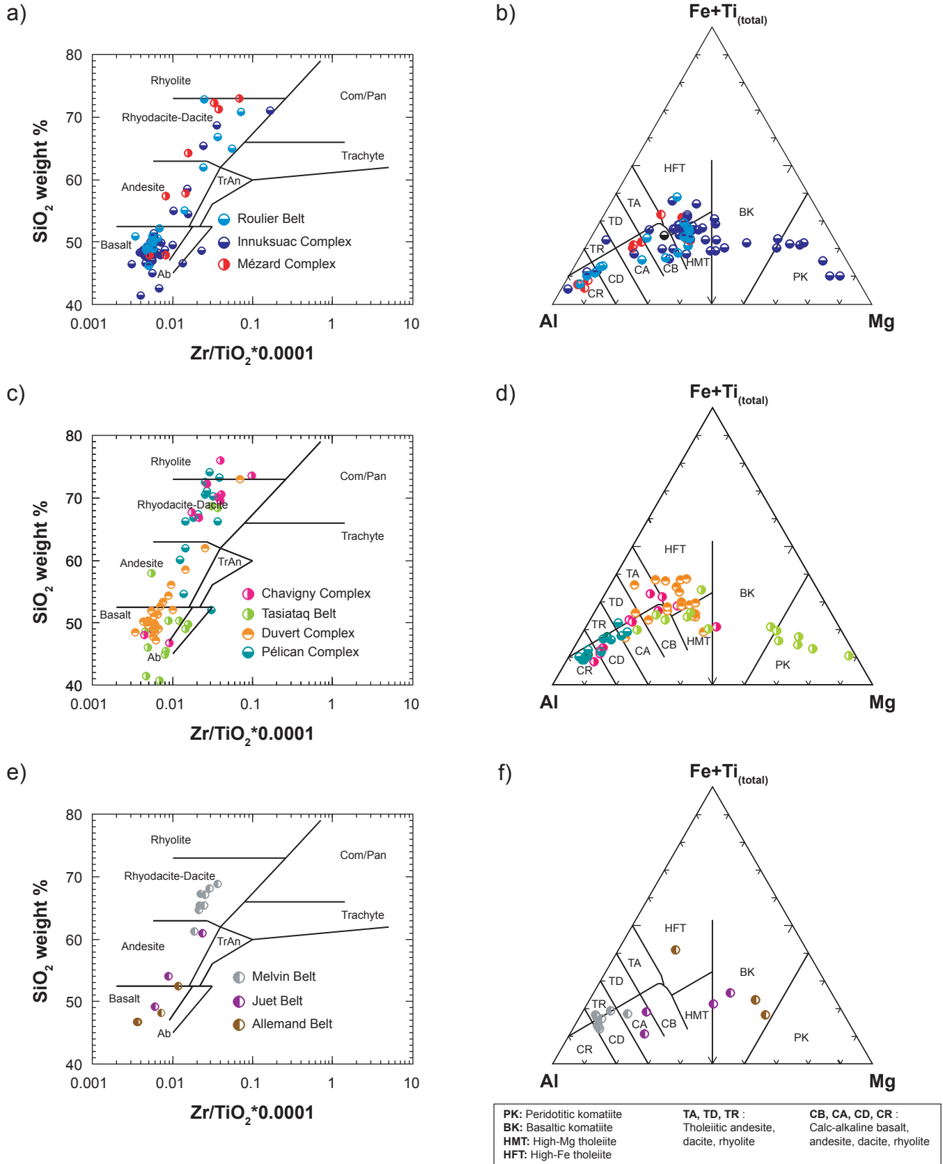
FIGURE 4.2 – Classification diagrams for volcanic rocks in the NESP (Innusuaq, Mézard, Chavigny, Duvert, and Pélican complexes and Roulier, Tasiataq, Melvin, Juet, and Allemand belts): a), c), and e) SiO 2 (weight %) vs Zr/TiO 2 *0.0001; b), d), and f) Jensen cation plot Mg–Al–Fe+Ti(total).
