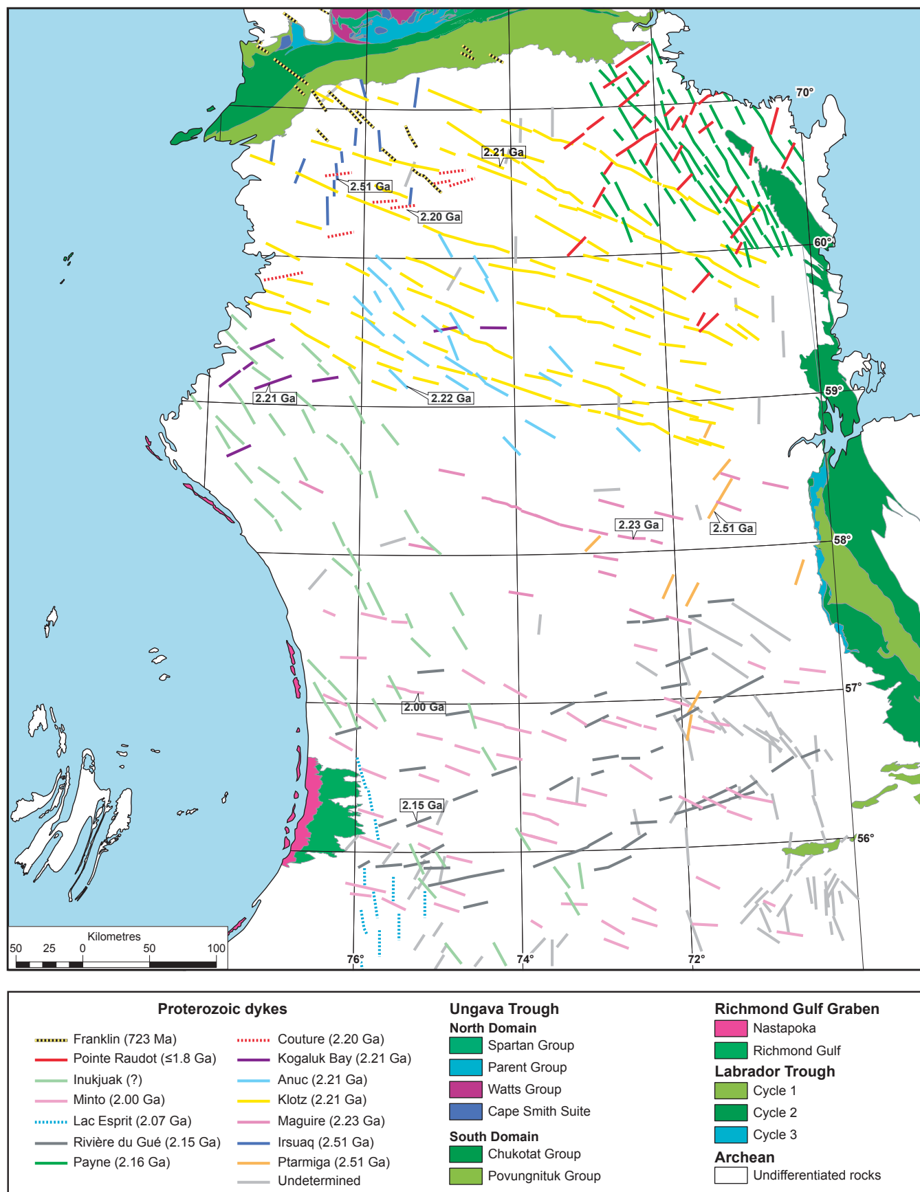
FIGURE 6.1 – Distribution of Proterozoic mafic dyke swarms in the northeastern Superior Province.
