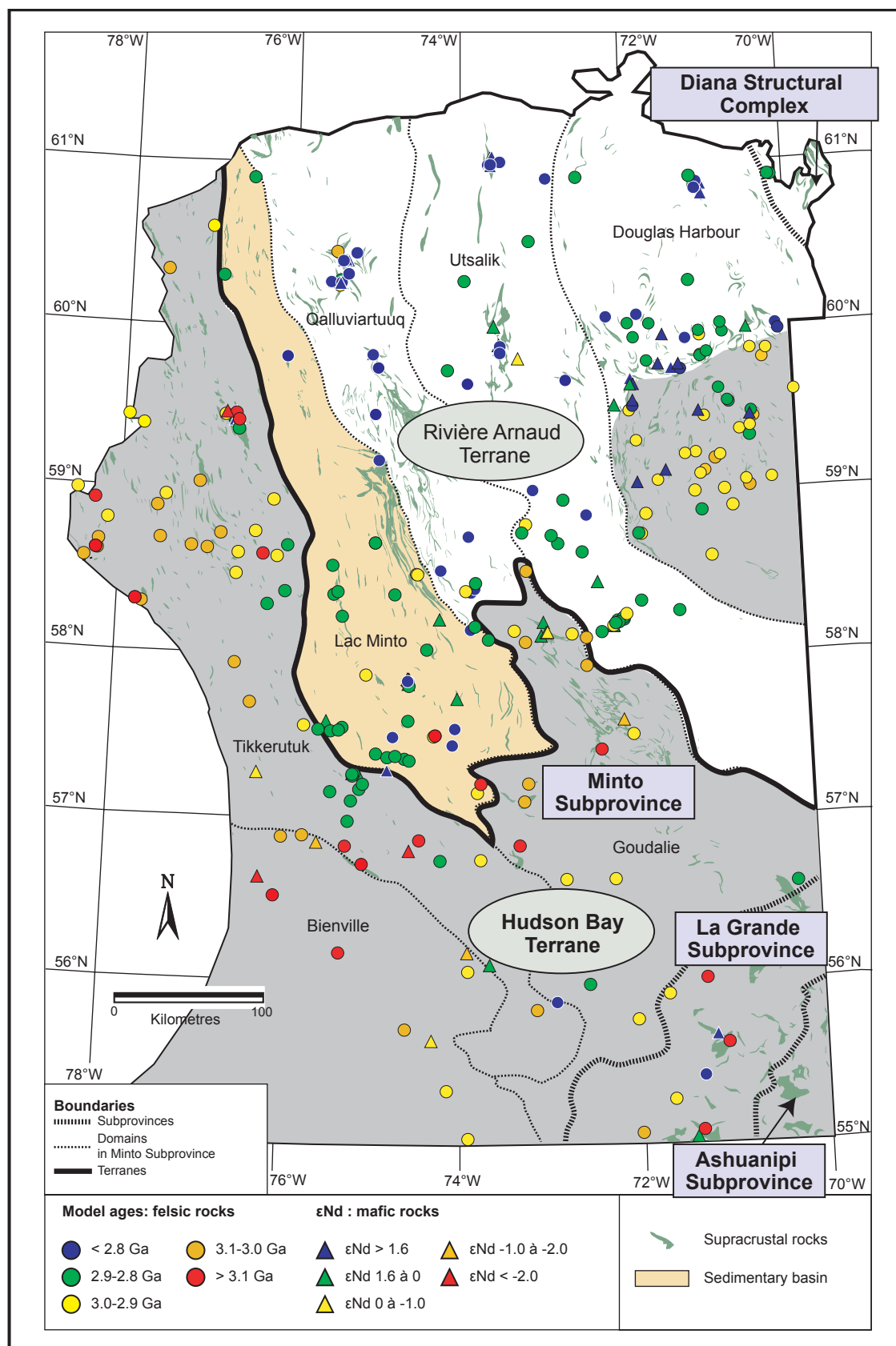
FIGURE 4.14 – Distribution of Nd isotope data in the NESP along with \epsilon\text{Nd}(t) values and mantle extraction model ages (TDM) (after Tomlinson et al. , 2004). Different coloured triangles refer to the \epsilon\text{Nd}(t) values (see legend) for mafic to ultramafic rocks or felsic to intermediate rocks with a ^{147}\text{Sm}/^{144}\text{Nd} ratio > 0.14. Different coloured circles refer to model ages (see legend) for felsic to intermediate rocks. Isotopic data come from different laboratories and are compiled in Table 4.4.
