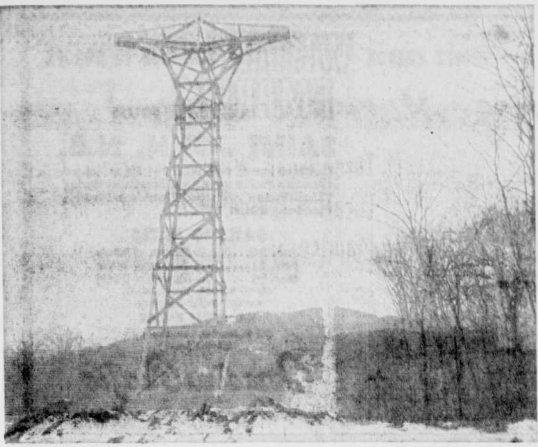
CANADA'S LONGEST CHAIR-LIFT — Pictured above is one of the fifteen frames at Mount Orford, which will carry Canada's longest chair-lift, scheduled to be completed by the end of this month. Designed particularly for skiers, the lift is 5,500 feet long. (Record photo by Charles Catchpaugh)
