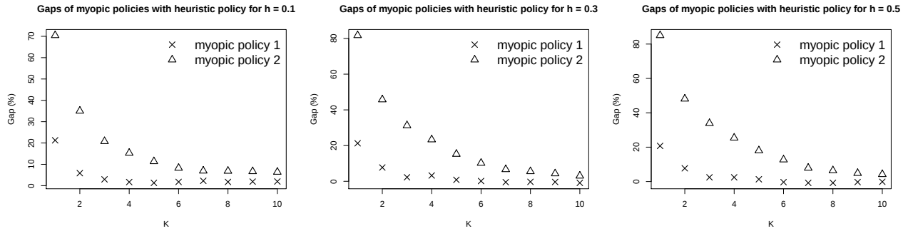
Figure 3: Objective gaps of myopic policies 1 and 2 compared to the heuristic policy for h = 0.1, 0.3, 0.5 .
