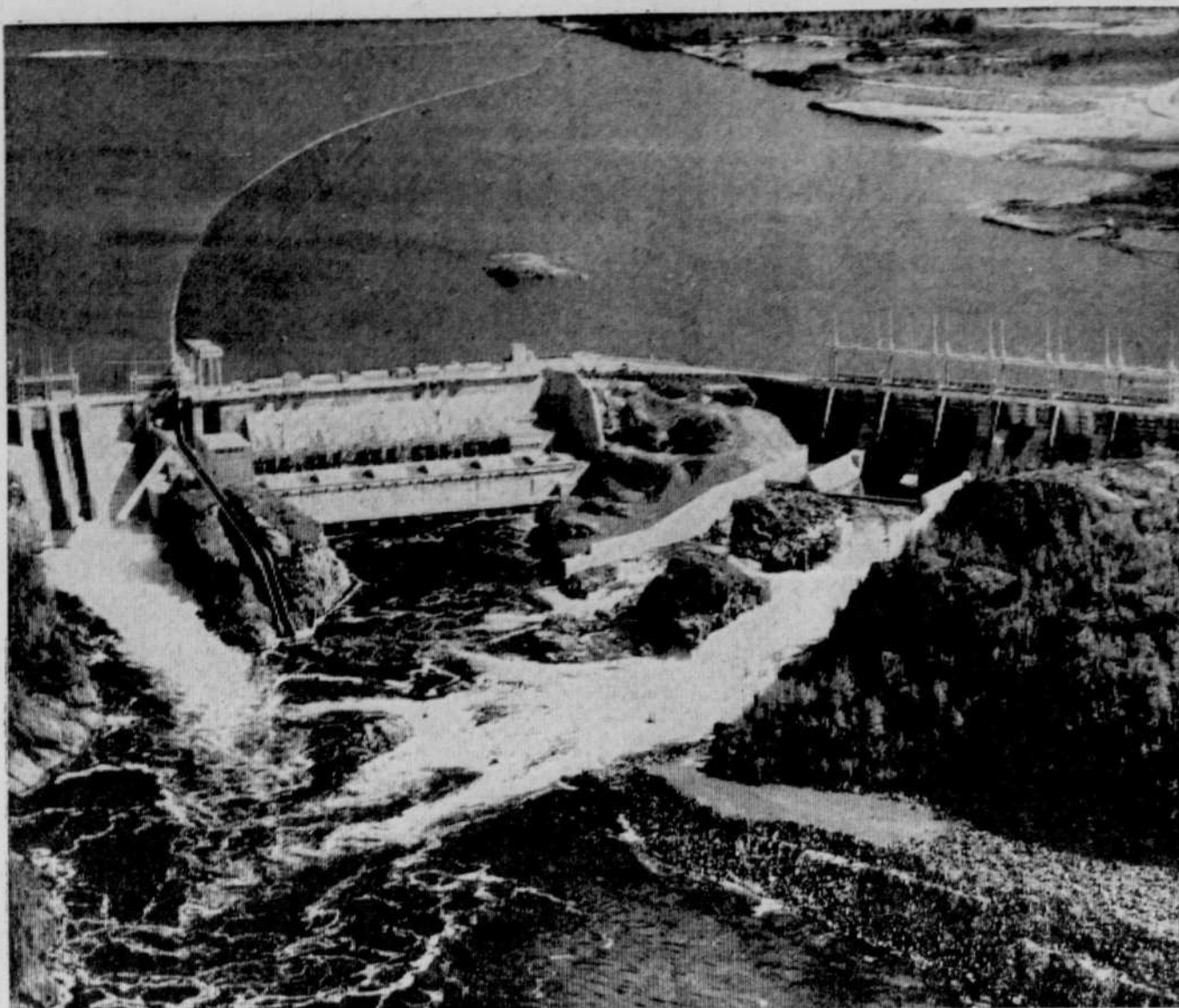
NOW GOVERNMENT OWNED — Saguenay Power Company, an affiliate of Aluminum Company of Canada is one of seven privately owned companies taken over recently by publicly-owned Quebec Hydro. Saguenay's Chute-du-Diable powerhouse, 1,920 feet long and 160 feet high above the lowest bedrock with an installed generating capacity of 275,000 horsepower, is on the Peribonca River, flowing into Lake St. John north of Quebec City. (CP Photo)
