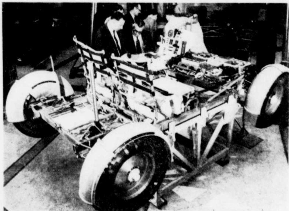
MOON BUGGY which will accompany Apollo 15 astronauts to the moon in July will resemble this model, assembled at Boeing's Kent Space Center near Seattle for qualification testing to NASA standards. The first manned self-propelled vehicle on the moon, the battery-powered Lunar Roving Vehicle (LRV) will provide a vastly superior equipment transporter to the hand-pulled cart used on the Apollo 14 mission. Diagram below shows principal features of the vehicle.
