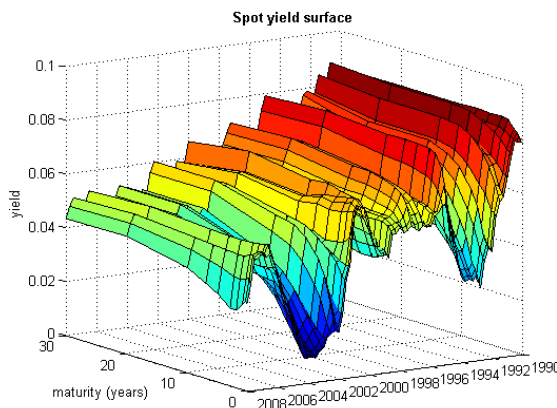
Figure 17: Spot-yield surface.
