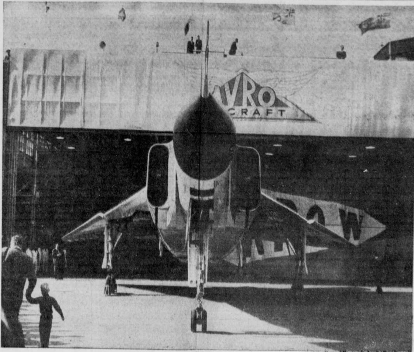
New Jet Plane — This is a nose-on view of CF-105 supersonic Arrow unveiled at the Avro Aircraft Ltd. plant in Toronto. The plane, which has not yet flown, is said to have a speed of 1,200 miles an hour and will be capable of carrying a hydrogen bomb. Because of its enormous thirst for fuel, however, it will be able to remain in the air only 20 to 30 minutes. (CP Photo)
