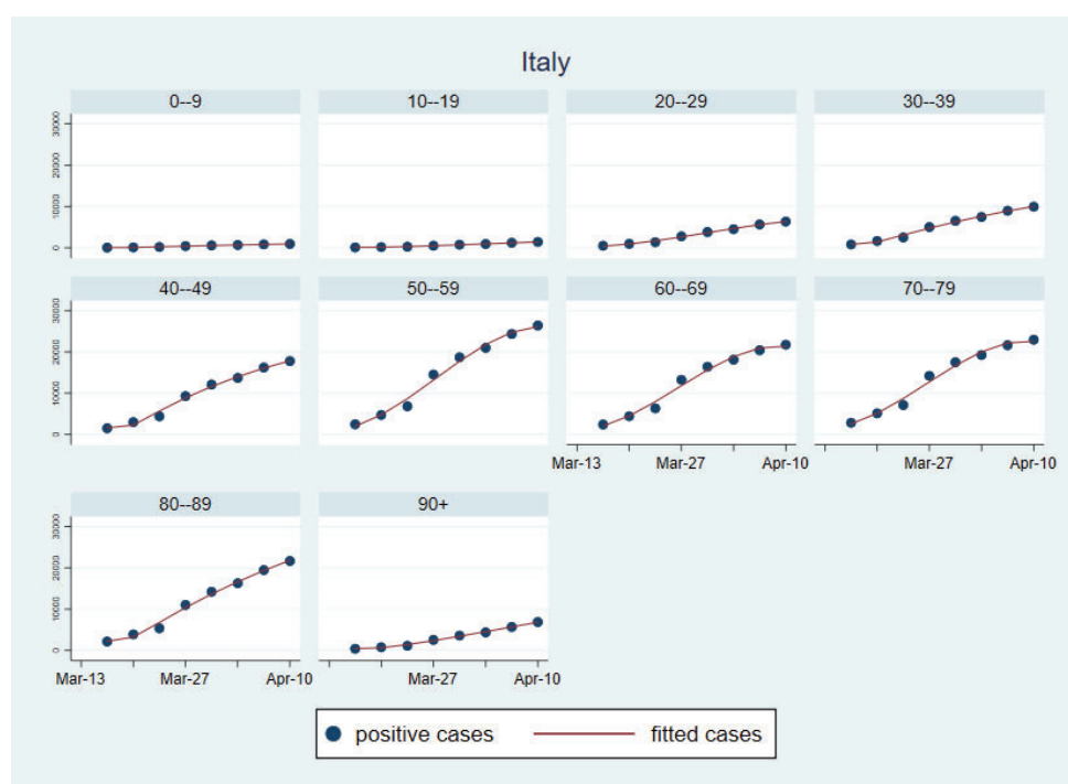
FIGURE 2. Cumulative number of confirmed positive cases, by age group
