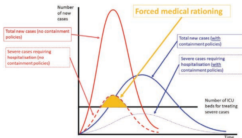
Figure 1. An illustration of “flattening the curve” of COVID-19 infections
