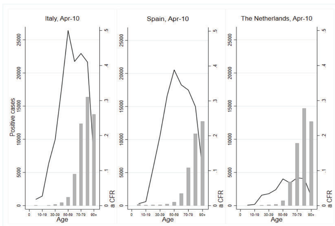
FIGURE 4. Number of confirmed positive cases and case-fatality risk, by age group
