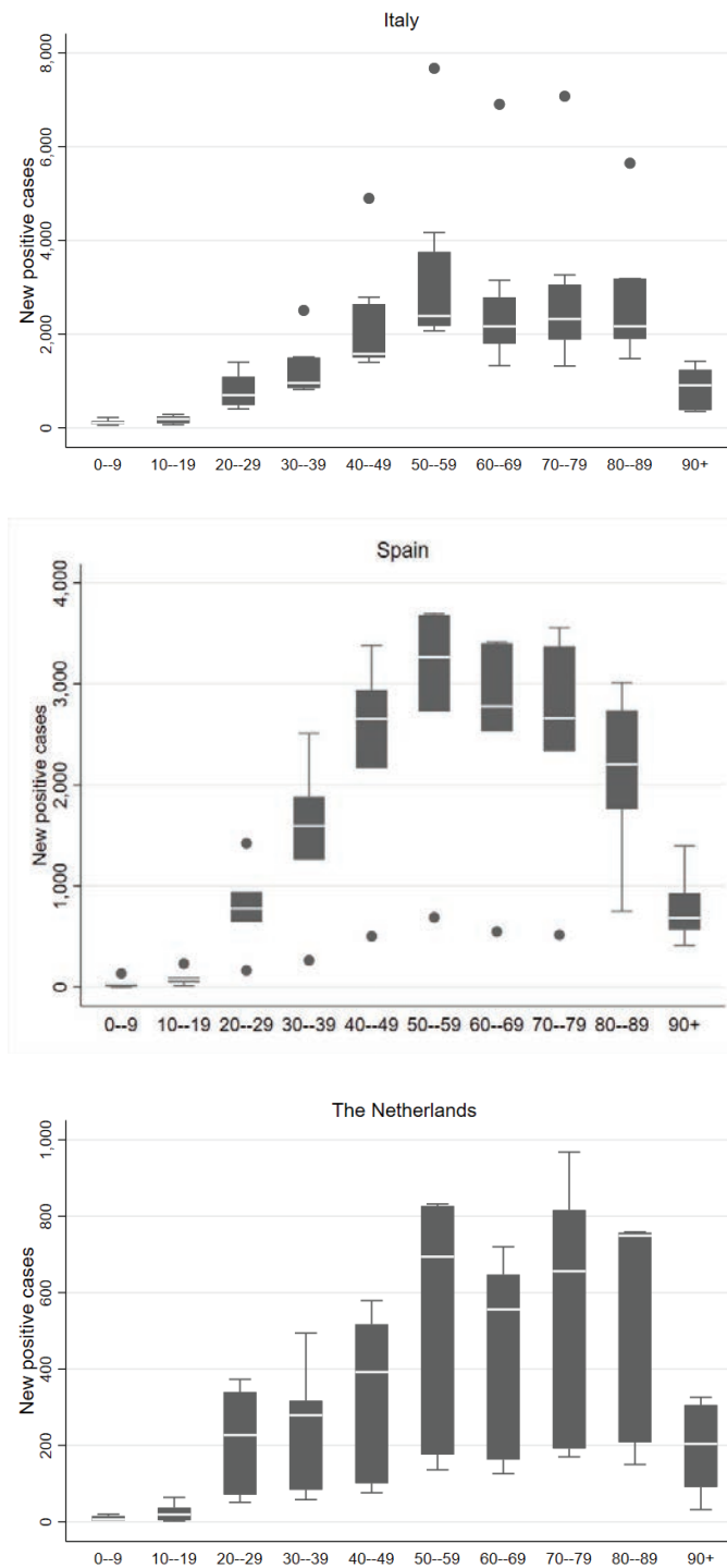
FIGURE 3. Increase in the number of confirmed positive cases, by age group
