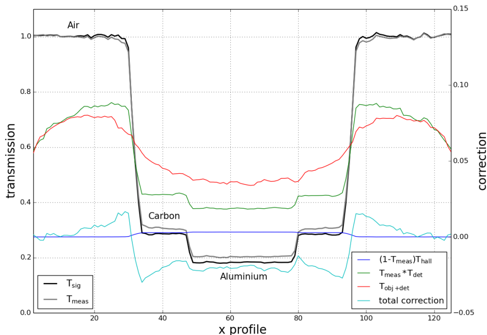
Figure 1 Illustrative example of the corrections applied to a given slice in the case of an object made of concentric cubes of carbon and aluminium.
