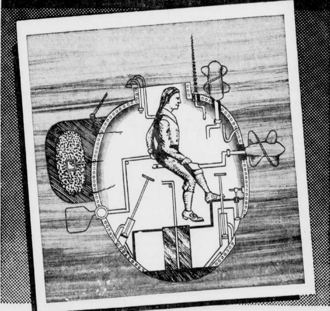
Submarine Turtle, 1776
