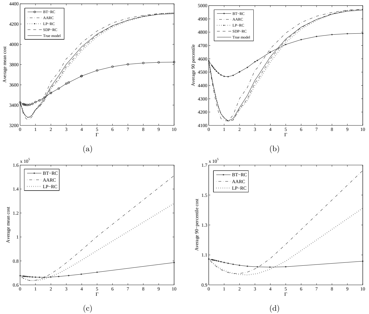
Figure 1: Average expected cost and average 90th percentile (over 1000 problem instances) achieved by robust solutions given different level of conservativeness. While Figure (a) presents average expected cost and Figure (b) presents average 90th percentile for a horizon of 10 periods, Figures (c) and (d) present the same statistics for a horizon of 100 periods.
