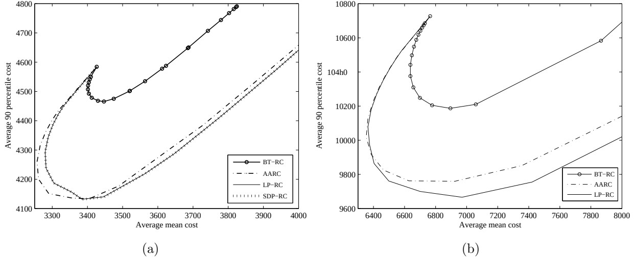
Figure 2: Average expected cost versus average 90th percentile achieved by the different robust methods when adjusting the level of conservativeness \Gamma . Figure (a) presents the achieved risk-return trade-offs for a 10 days horizon while (b) presents it for a 100 days horizon.
