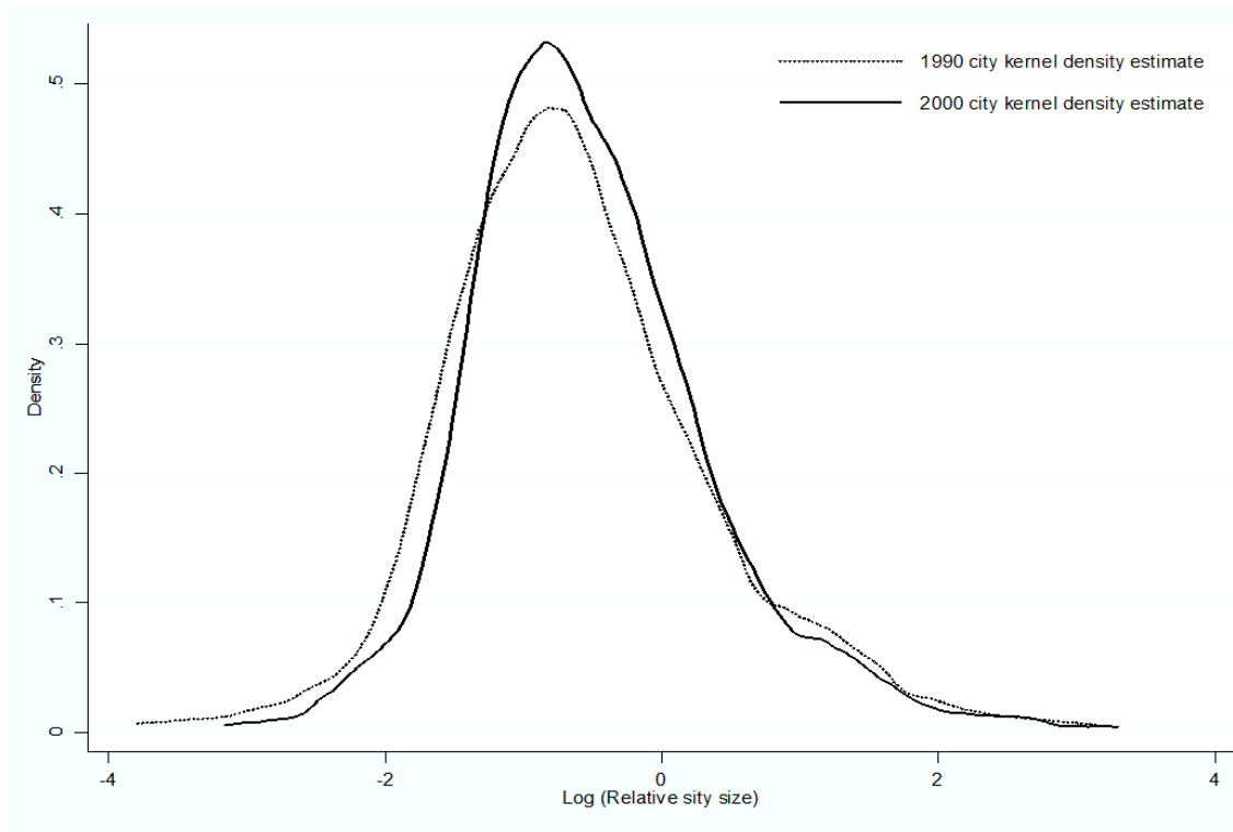
Figure. 2. Kernel density estimate of city size distribution, 1990 and 2000.
