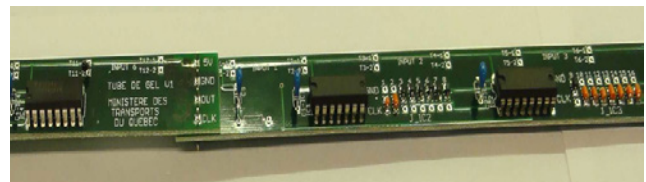
Figure 2: Overview of printed circuits of the electronic frost depth probe
