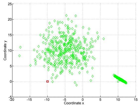
Figure 4: Non-cooperative case with high social effect ( q = 40 ). The population reaches consensus on p_2 .
