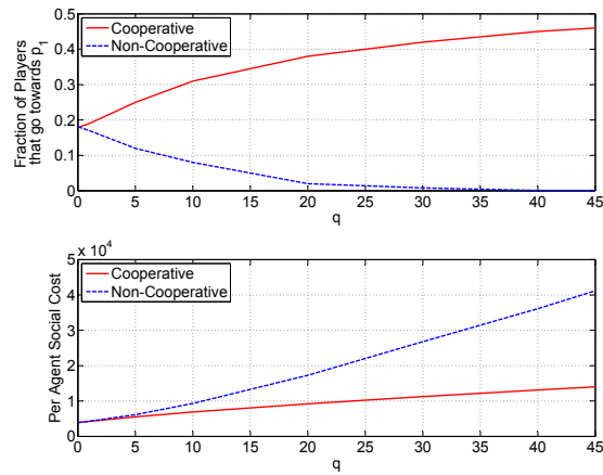
Figure 1: Cooperative vs. non-cooperative behavior.
