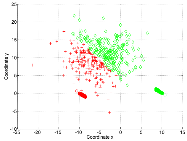
Figure 3: Cooperative case with high social effect ( q = 40 ). The population splits more evenly.
