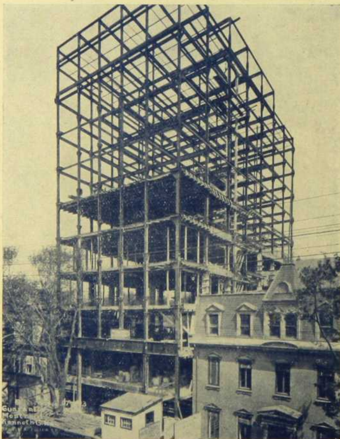
10 storey building for the Guarantee Co. of North America—Montreal. Steel frame erected in 24 working days.
