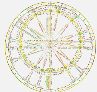
Theoria Solis per Ezechirum Sine Epiphora | Celestial Atlas of Andreas Cellarius 1661
