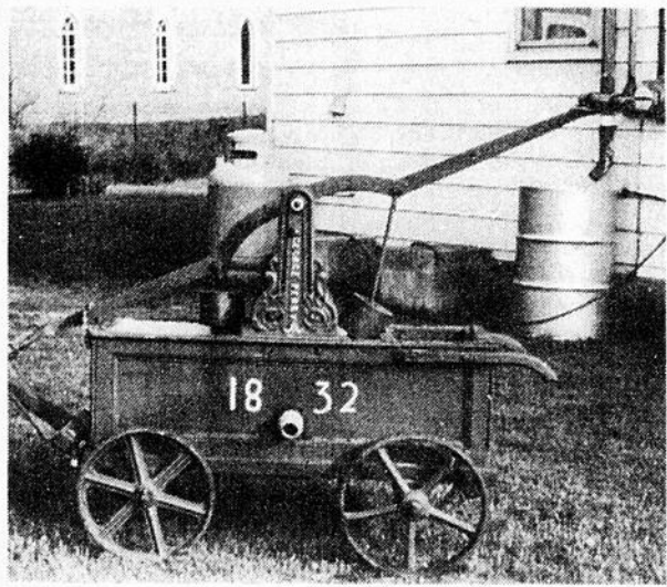
One of the oldest pieces in the museum is an 1832 George Perry Fire Tub Pump bought from a Napierville Fire Department. A bucket brigade filled the tub with water while two men pumped the water through a hose that was attached on the side of the tub, onto the fire.
