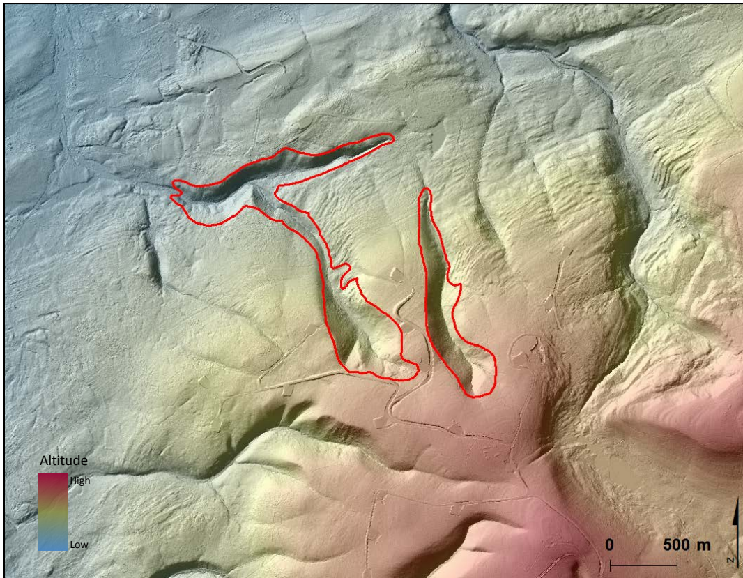
Figure 73. Example of colluviums (8c), on LiDAR, in the Eastern Balsam Fir-White Birch ecozone
