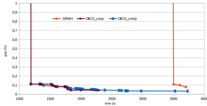
Figure 8: Gap evolution for DICG and DRMH for CPP_320 test
