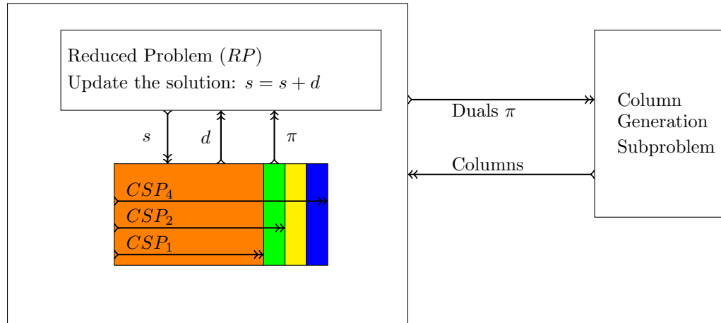
Figure 4: Column generation in IVD mode for q'=4
