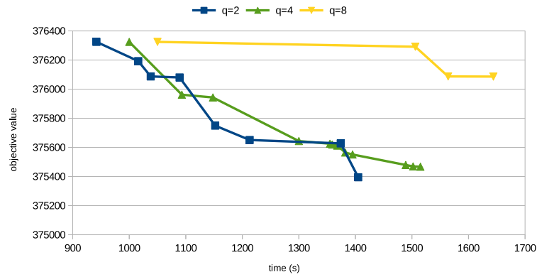
Figure 5: Influence of q on CPP_319 during the DVD phase
