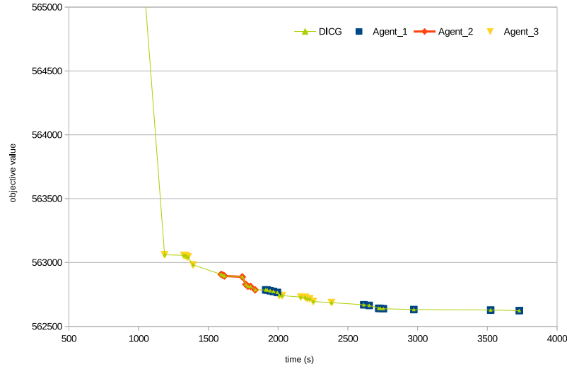
Figure 6: DICG_{comp} evolution over time on CPP_320
