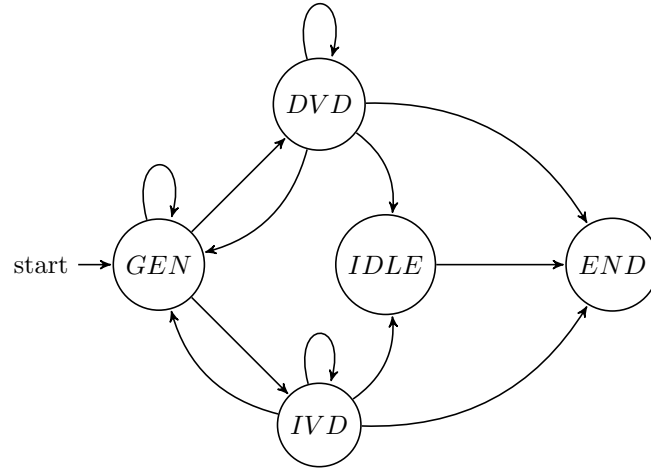
Figure 2: Worker agent basic state evolution
