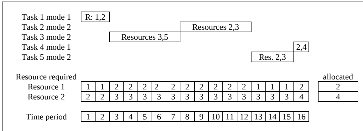
Figure 3: Optimal solution of the RACP
