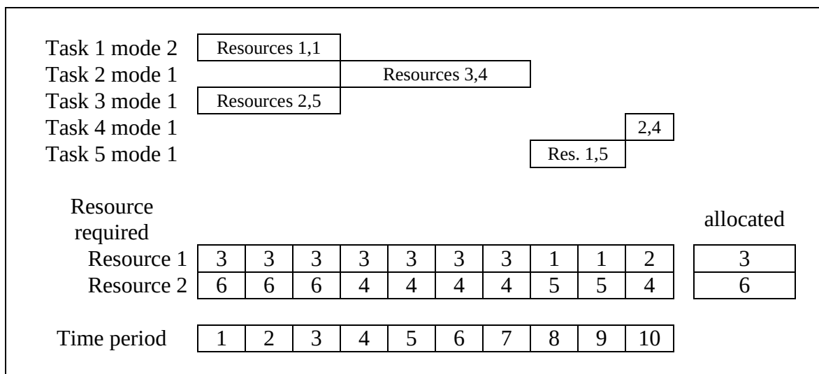
Figure 2: Optimal solution of the GRALP
