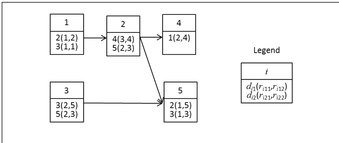
Figure 1: the 5-task, 2-resource numerical example
