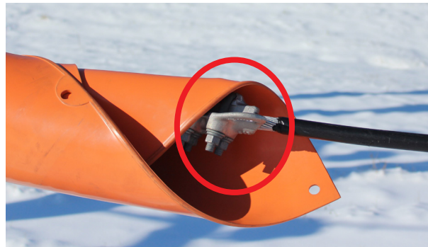
Part of the conductor is exposed
