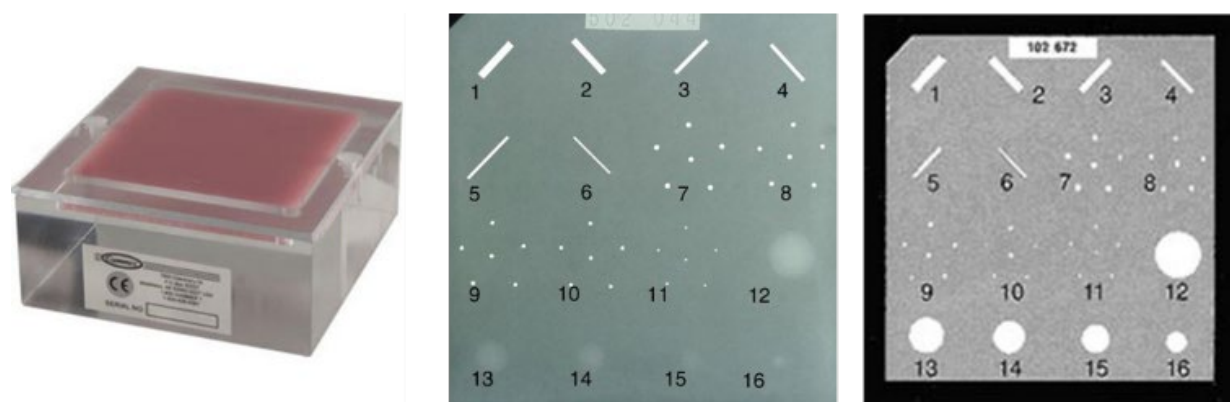
Figure 2 Fantôme RMI-156
