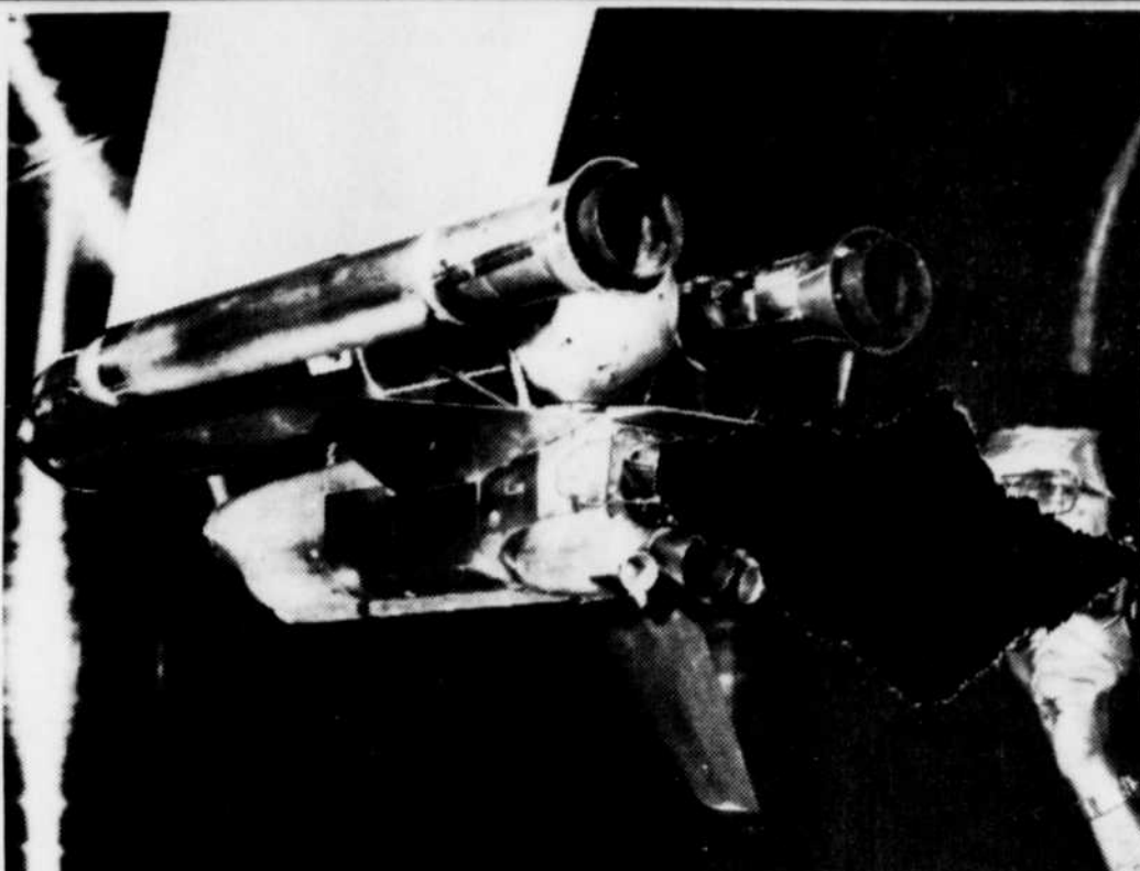
MINI-SCALE SPACE SHUTTLE goes through wind tunnel tests at NASA's Lewis Research Center in Cleveland in a trial run for the real thing. The model, equipped with hydrogen-oxygen engines and solid-propellant rocket motors, was mounted upside down to accommodate attachment hardware in the tunnel which operates at from 2 to 3.5 times the speed of sound.
