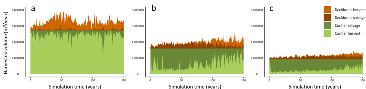
Figure 18. Annual conifer (in green) and deciduous (in orange) volume harvested over the 150-year simulation period with status quo forest management under (a) historical, (b) RCP 4.5, and (c) RCP 8.5 climates. Volumes salvaged after fire are represented in a darker shade (dark green for conifer and dark orange for deciduous volumes).
