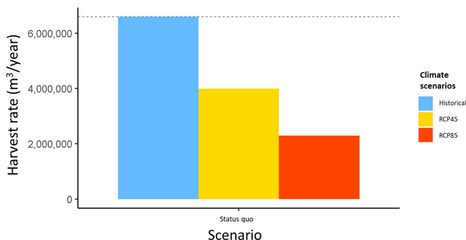
Figure 17. Maximum sustained yield harvest rates obtained for the status quo management scenario under the historical, RCP 4.5, and RCP 8.5 climate scenarios.
