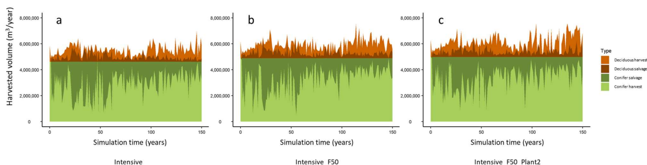
Figure 27. Annually harvested volumes under the (a) Intensive, (b) Intensive_F50, and (c) Intensive_F50_Plant2 adaptation scenarios.
