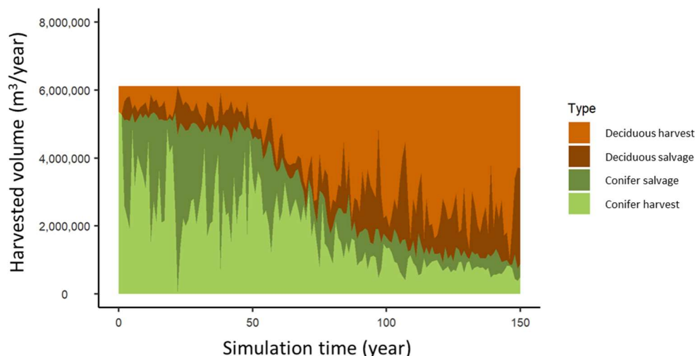
Figure 23. Harvested volumes under the deciduous enrichment scenario over the 150-year simulation period, under the RCP 4.5 climate scenario.
