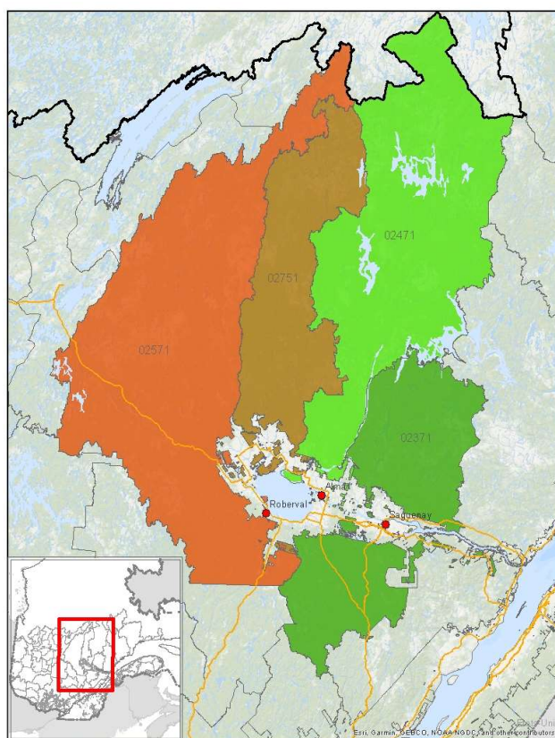
Figure 4. Location of the study area, in the Saguenay – Lac-Saint-Jean area.
