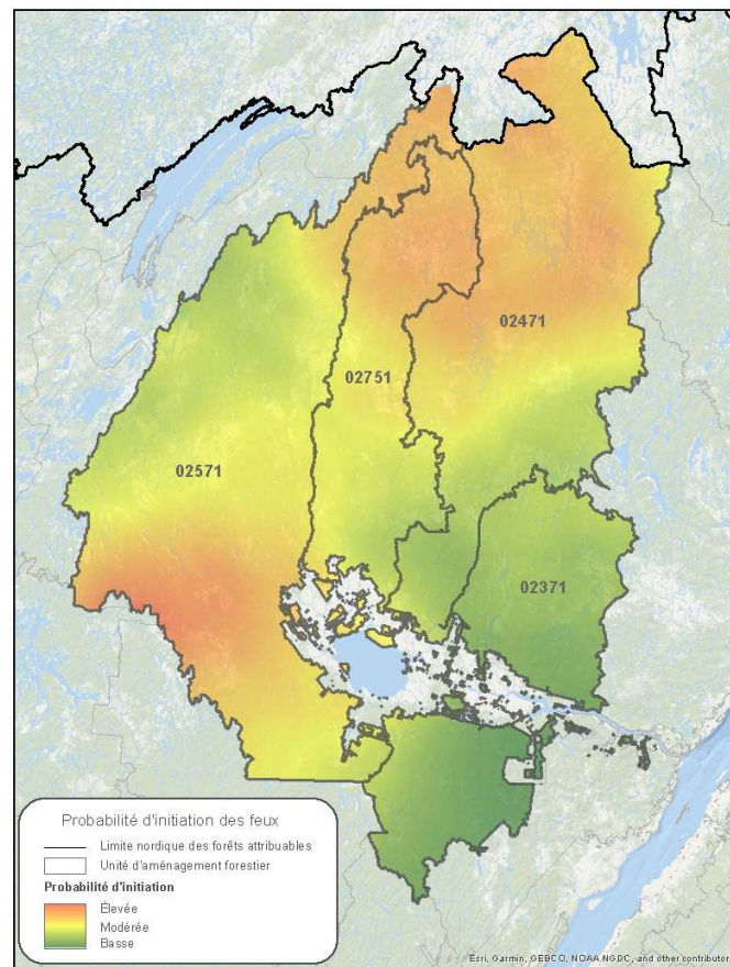
Figure 5. Probability of initiation of wildfires over the region.
