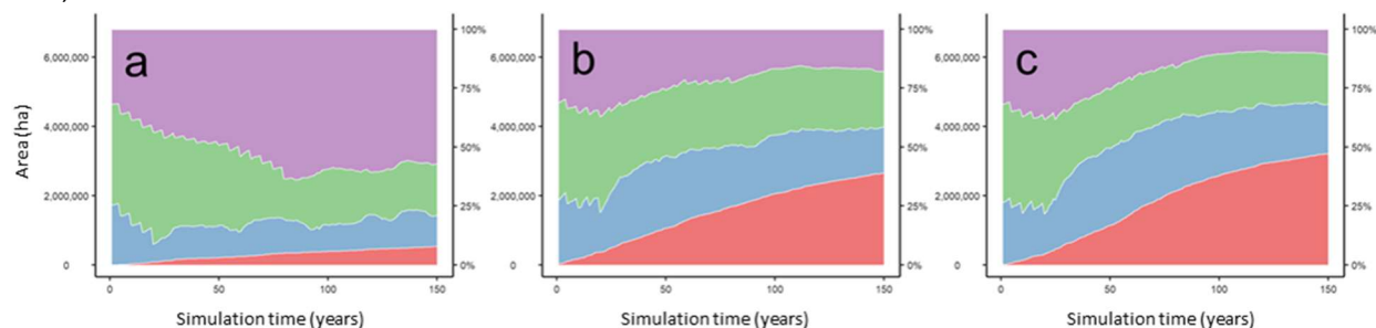
Figure 12. Diagrams illustrating the abundance of age classes without forest management under (a) the historical climate, (b) RCP 4.5, and (c) RCP 8.5. Area as regeneration failure is shown in red, regenerating area is shown in blue, premature and mature forest is in green, and old forest is shown in violet.
