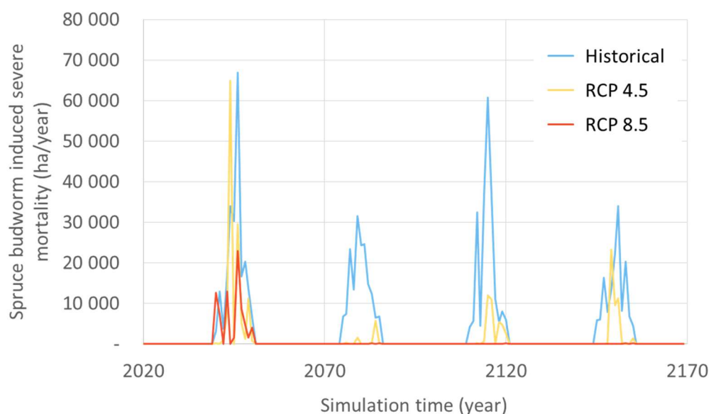
Figure 16. Area affected annually by severe mortality due to spruce budworm defoliation under the three climate scenarios.
