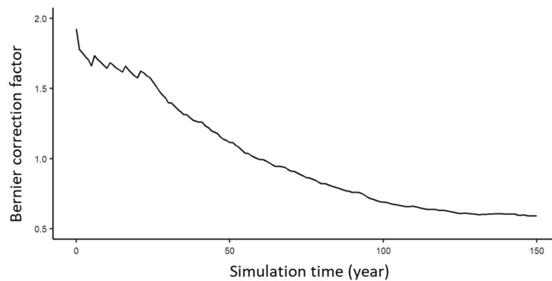
Figure 24. Evolution of the Bernier et al. (2016) correction factor while simulating the deciduous enrichment scenario and the RCP 4.5 climate scenario. A higher correction factor leads to a greater annual area burned. A correction factor of 1 corresponds to a burn rate from which the effect of forest composition has been removed (section 3.2.4.1).
