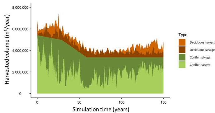
Figure 30. Adjustment of harvest rates over time, seeking to stabilize timber supply over the long term. These results were obtained with the Intensive_F50_Plant2 adaptation scenarios under the RCP 8.5 climate scenario.
