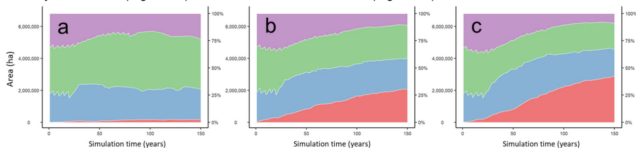
Figure 20. Diagrams illustrating the abundance of age classes for status quo management under (a) the historical climate, (b) RCP 4.5, and (c) RCP 8.5. Area as regeneration failure is shown in red, regenerating area is shown in blue, premature and mature forest is in green and old forest is shown in violet.
