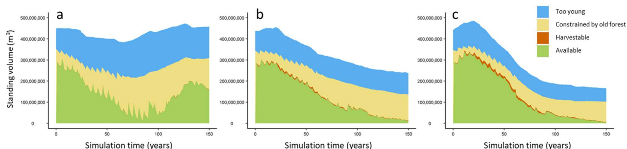
Figure 19. Standing volume in the study area under the status quo management scenario under the (a) historical, (b) RCP 4.5, and (c) RCP 8.5 scenarios. Volumes that are available for harvest are shown in green (live trees) and orange (salvage).
