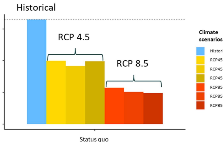
Figure 11. Illustration of the divergence of results from different climate scenarios (RCP) and convergence among results for different earth system models (ESM) but for the same climate scenario.
