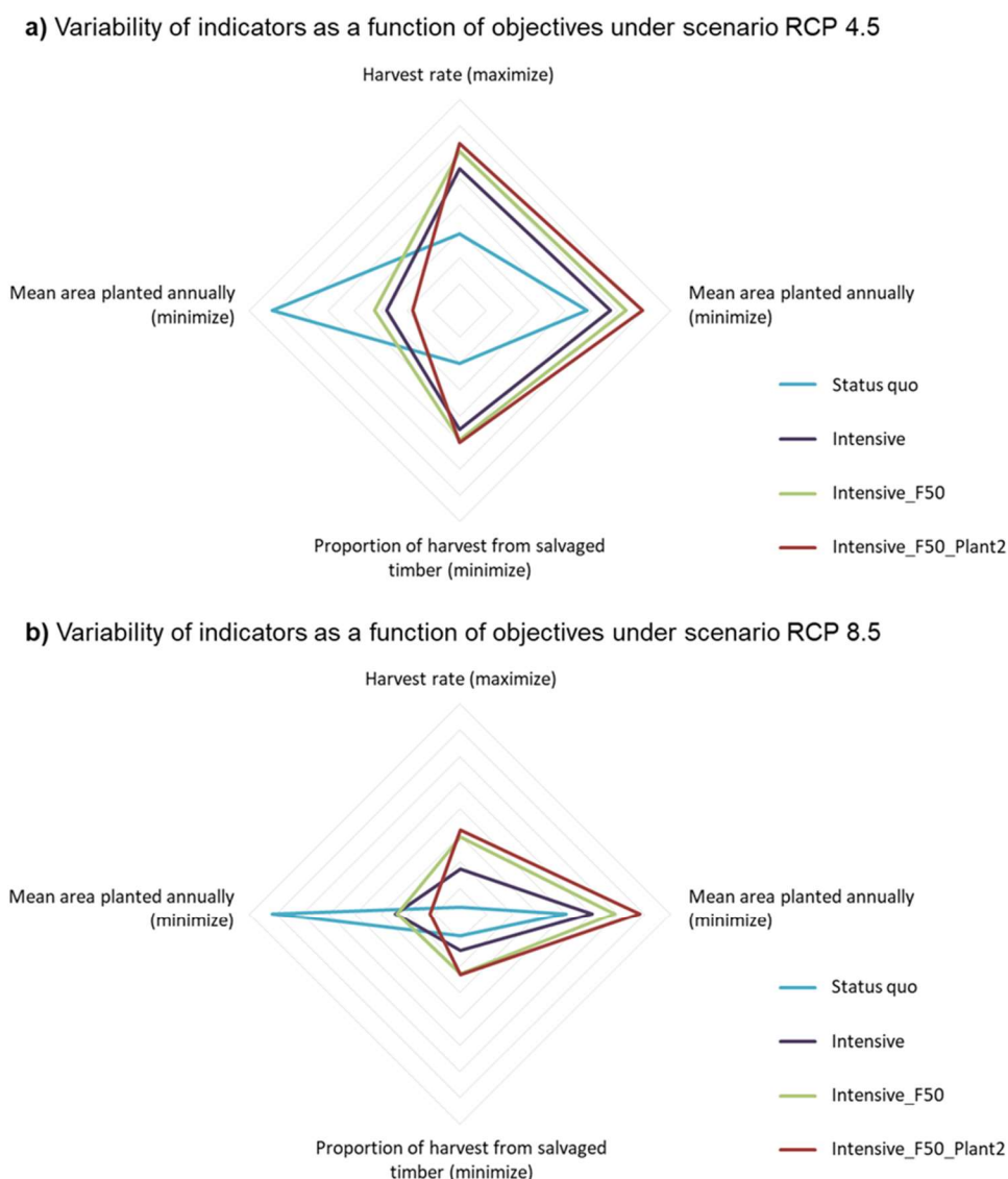
Figure 33. Variation of indicators according to the adaptation scenarios tested under (a) RCP 4.5 and (b) RCP 8.5.
