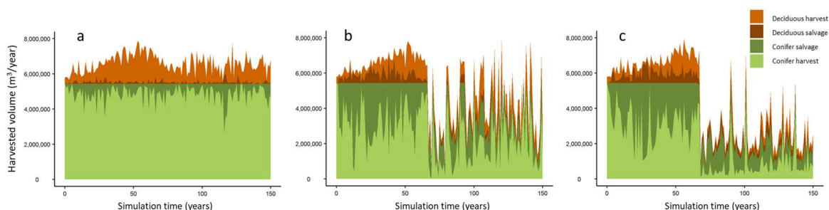
Figure 22. Annually harvested volumes under the status quo management scenario, under the (a) historical, (b) RCP 4.5, and (c) RCP 8.5 scenarios. The harvest rate under the historical climate is the maximum sustained yield harvest level. The harvest levels under RCP 4.5 and RCP 8.5 is the maximum sustained yield harvest level obtained under a historical climate, while allowing harvesting shortfalls to occur when sufficient wood volumes are not available in a given time period.
