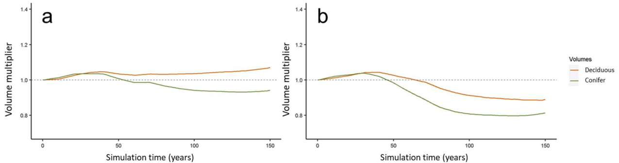
Figure 14. Mean values of merchantable volume multipliers (weighted by area) over 150 years of simulation for the status quo scenario under (a) RCP 4.5 et (b) RCP 8.5 for conifer (in green) and deciduous (in orange) merchantable volumes. The dotted horizontal line indicates a multiplier, equal to 1, under a historical climate.
