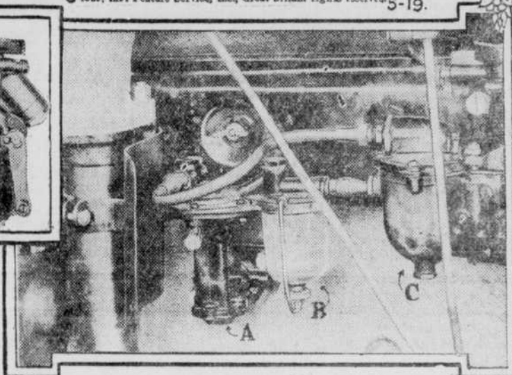
FUEL PUMP SYSTEM USED ON MODERN CAR. A, FUEL PUMP, B, STRAINER, C, CARBURETOR.
