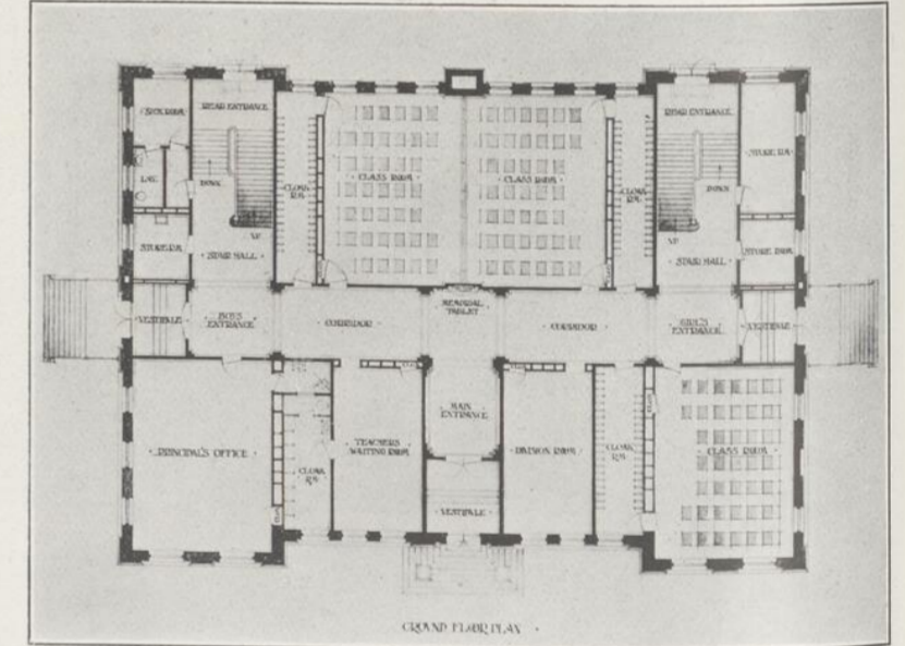
PROGRESS IN SCHOOL CONSTRUCTION: A 20th CENTURY CANADIAN EDIFICE —Interior plan of the ground floor in the Sarah Maxwell Memorial and Earl Grey Schools, Montreal.
