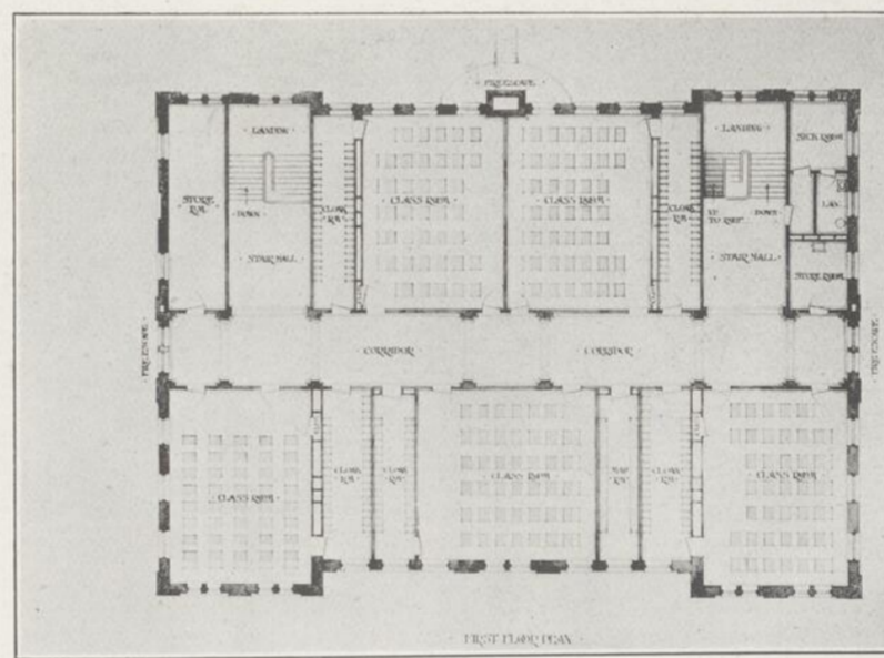
PROGRESS IN SCHOOL CONSTRUCTION: A 20th CENTURY CANADIAN EDIFICE —Interior plan of the first floor in the Sarah Maxwell Memorial and Earl Grey Schools, Montreal.
