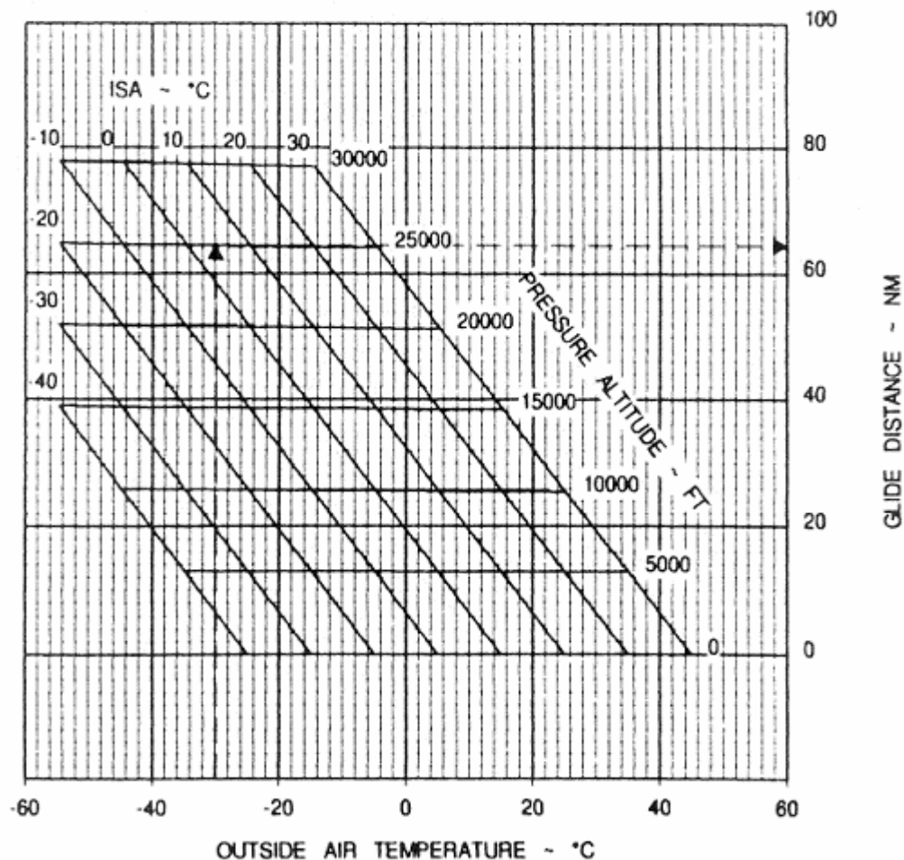
Figure 4.7 : Performances de planage du PC-12 [4.15]
