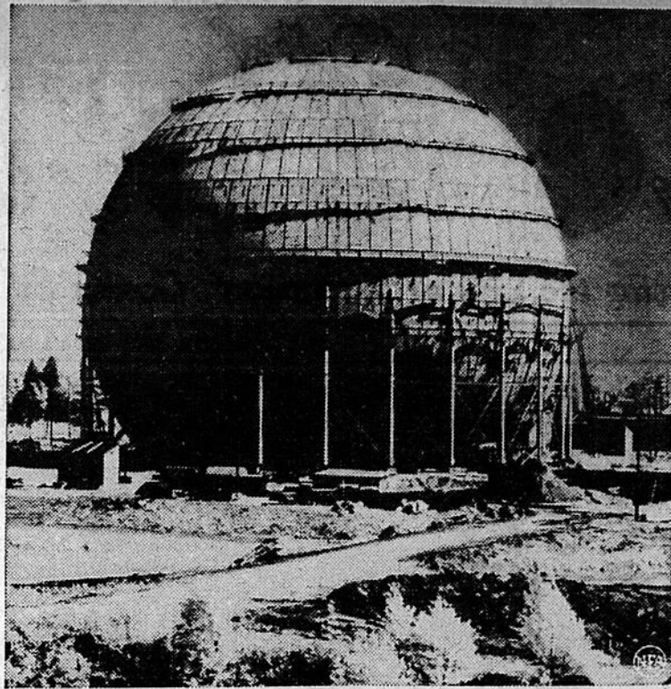
WORLD'S BIGGEST BALL: This huge sphere, at Schenectady, N.Y., said to be the largest in the world (3850 tons of steel), is ready to house the prototype of an atomic power plant for submarines. Inch thick steel plates are joined together by more than five miles of welding to make ball as high as an 18-story building.
