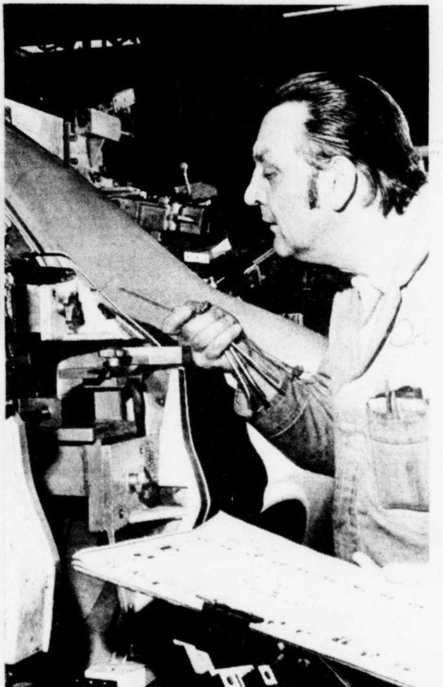
supervisor uses a "Mintect" to measure the thickness of paint on a light truck. At right, a quality control inspector uses a metal "feeler" gauge to check dimensions of a car before it continues along the assembly line. With one quality control inspector for every nine assemblers quality control personnel follow cars and trucks from the body build through final assembly.
